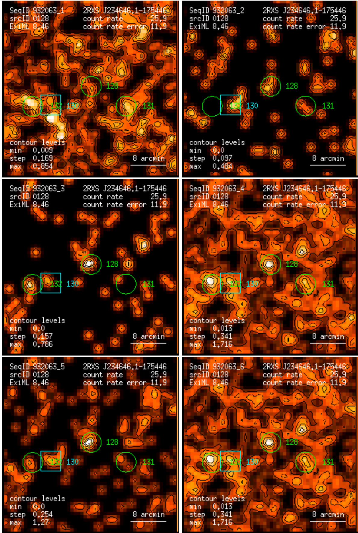
Figure 128: RASS 932063: detection 0128: band rate images, Gaussian filter: (1) PSPC channels 11 – 41, (2) 52 – 90, (3) 91 – 201, (4) 11 – 235, (5) 52 – 201, (6) 11 – 201. Broad band rates in counts/ks. Band rate contour levels in counts/ks/arcmin 2 .
