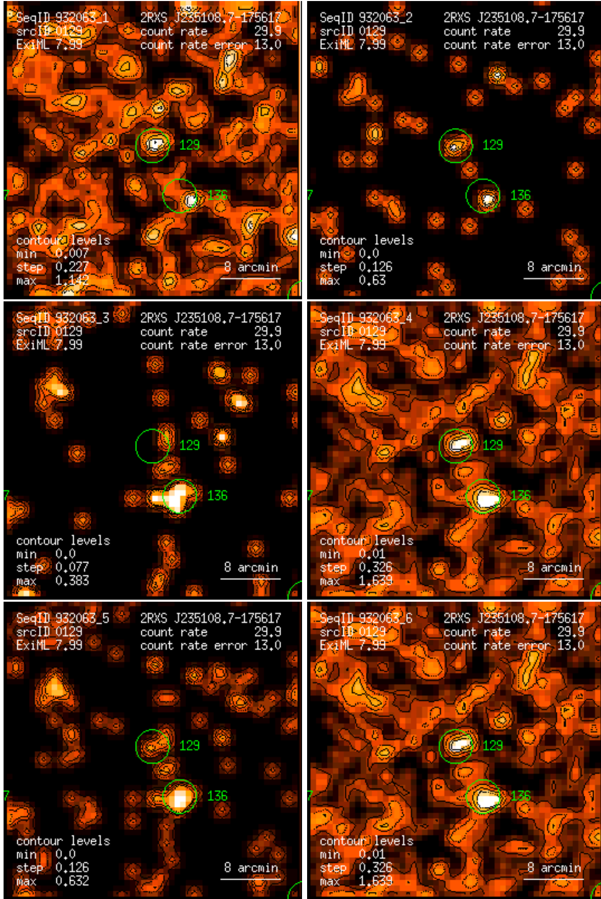
Figure 129: RASS 932063: detection 0129: band rate images, Gaussian filter: (1) PSPC channels 11 – 41, (2) 52 – 90, (3) 91 – 201, (4) 11 – 235, (5) 52 – 201, (6) 11 – 201. Broad band rates in counts/ks. Band rate contour levels in counts/ks/arcmin 2 .
