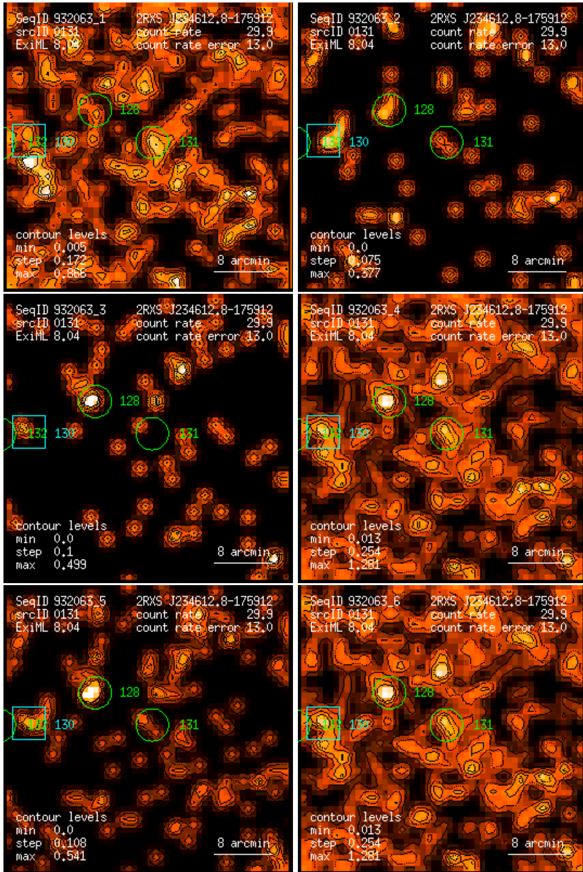
Figure 131: RASS 932063: detection 0131: band rate images, Gaussian filter: (1) PSPC channels 11 – 41, (2) 52 – 90, (3) 91 – 201, (4) 11 – 235, (5) 52 – 201, (6) 11 – 201. Broad band rates in counts/ks. Band rate contour levels in counts/ks/arcmin 2 .
