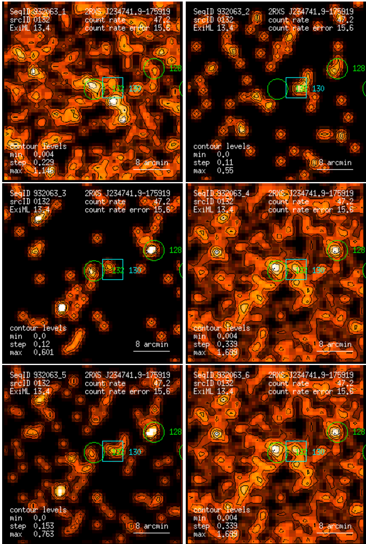
Figure 132: RASS 932063: detection 0132: band rate images, Gaussian filter: (1) PSPC channels 11 – 41, (2) 52 – 90, (3) 91 – 201, (4) 11 – 235, (5) 52 – 201, (6) 11 – 201. Broad band rates in counts/ks. Band rate contour levels in counts/ks/arcmin 2 .
