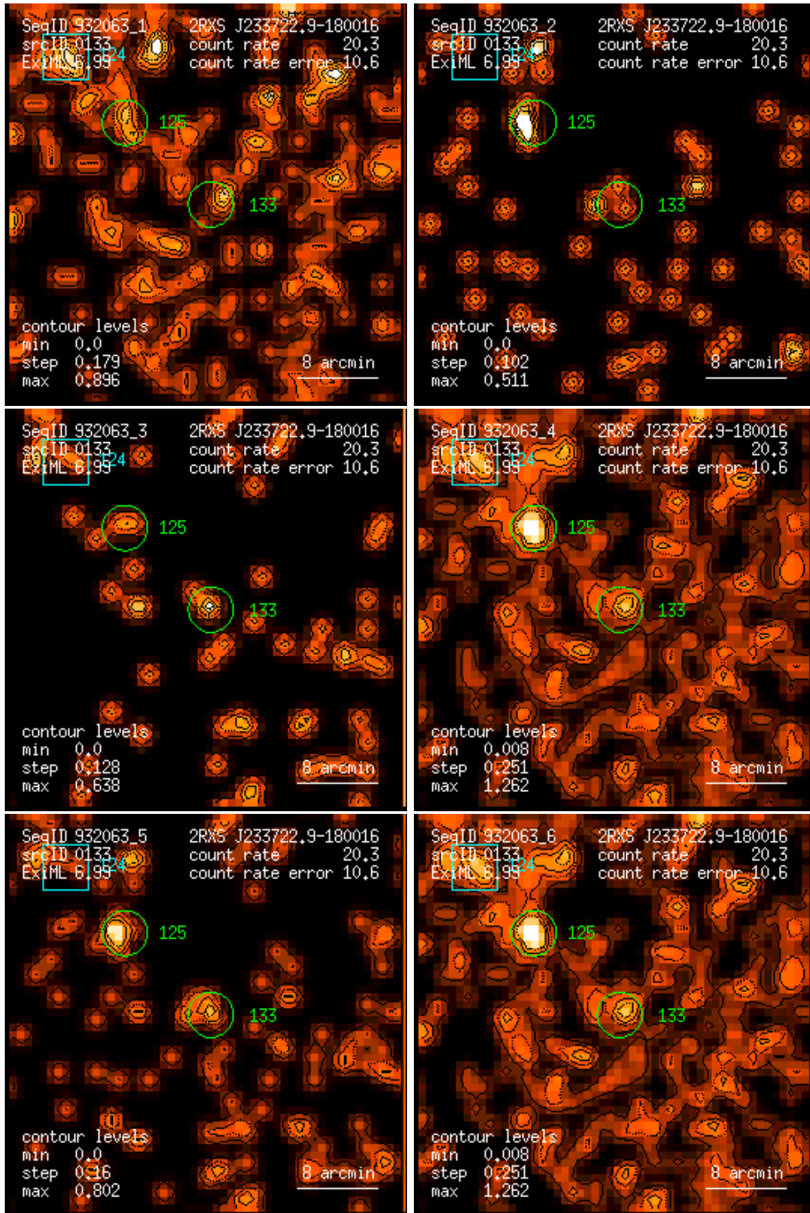
Figure 133: RASS 932063: detection 0133: band rate images, Gaussian filter: (1) PSPC channels 11 – 41, (2) 52 – 90, (3) 91 – 201, (4) 11 – 235, (5) 52 – 201, (6) 11 – 201. Broad band rates in counts/ks. Band rate contour levels in counts/ks/arcmin 2 .
