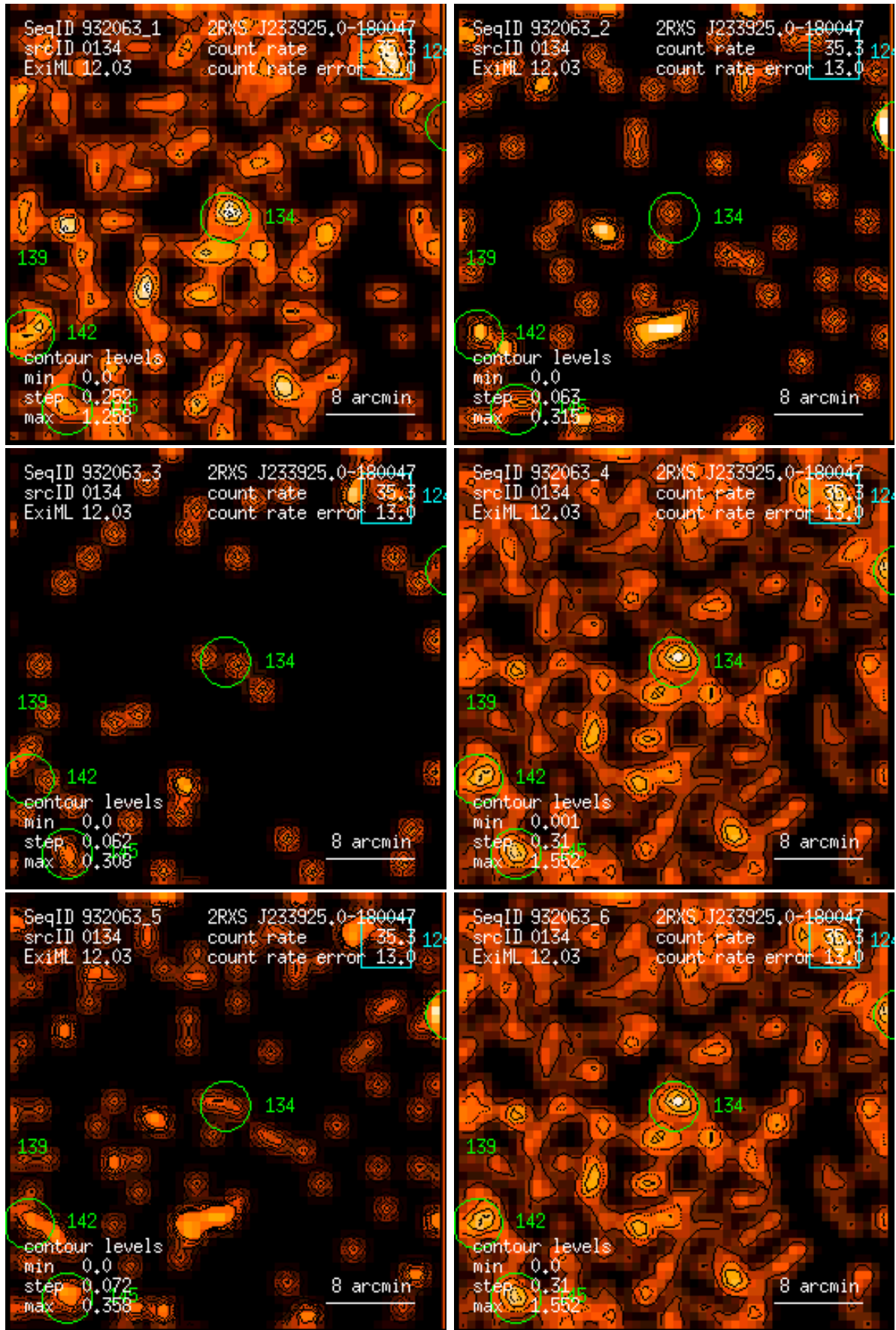
Figure 134: RASS 932063: detection 0134: band rate images, Gaussian filter: (1) PSPC channels 11 – 41, (2) 52 – 90, (3) 91 – 201, (4) 11 – 235, (5) 52 – 201, (6) 11 – 201. Broad band rates in counts/ks. Band rate contour levels in counts/ks/arcmin 2 .
