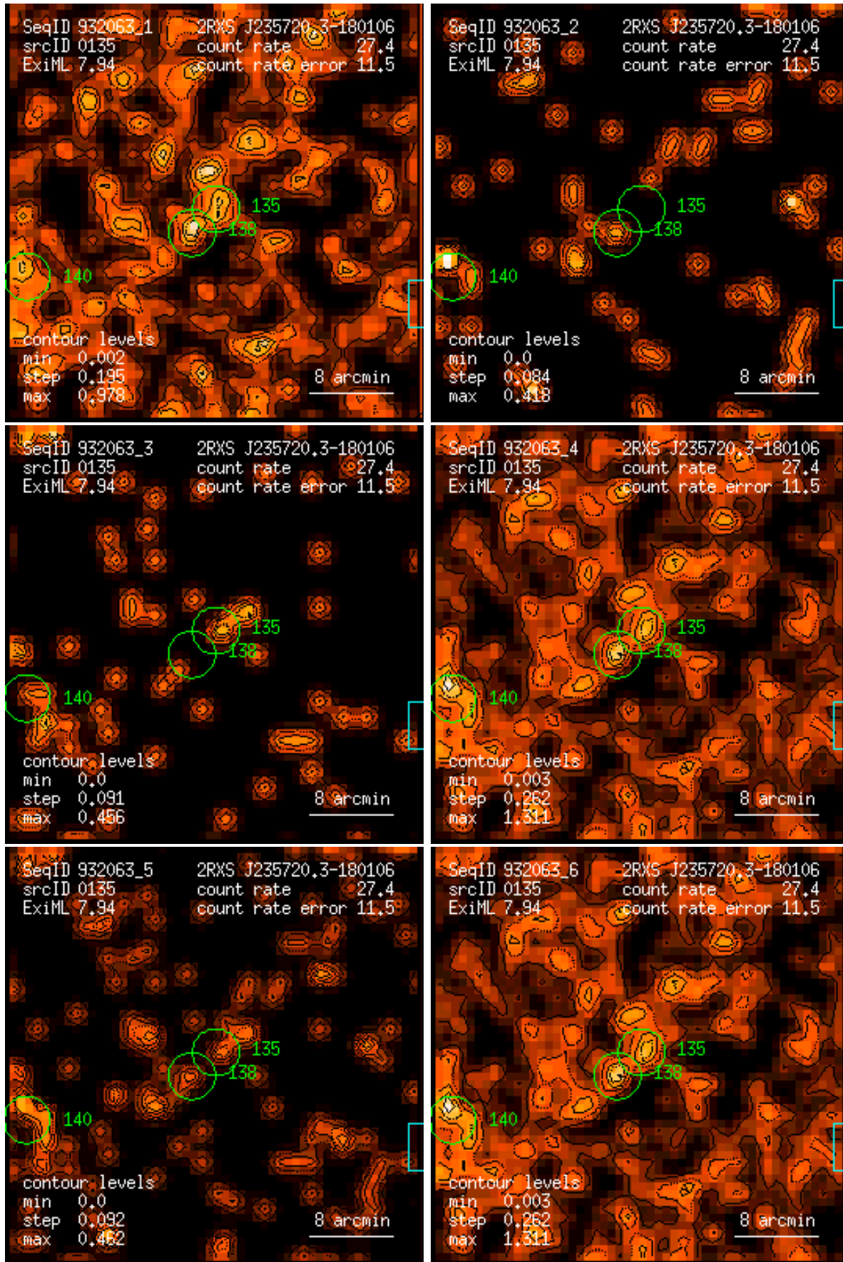
Figure 135: RASS 932063: detection 0135: band rate images, Gaussian filter: (1) PSPC channels 11 – 41, (2) 52 – 90, (3) 91 – 201, (4) 11 – 235, (5) 52 – 201, (6) 11 – 201. Broad band rates in counts/ks. Band rate contour levels in counts/ks/arcmin 2 .
