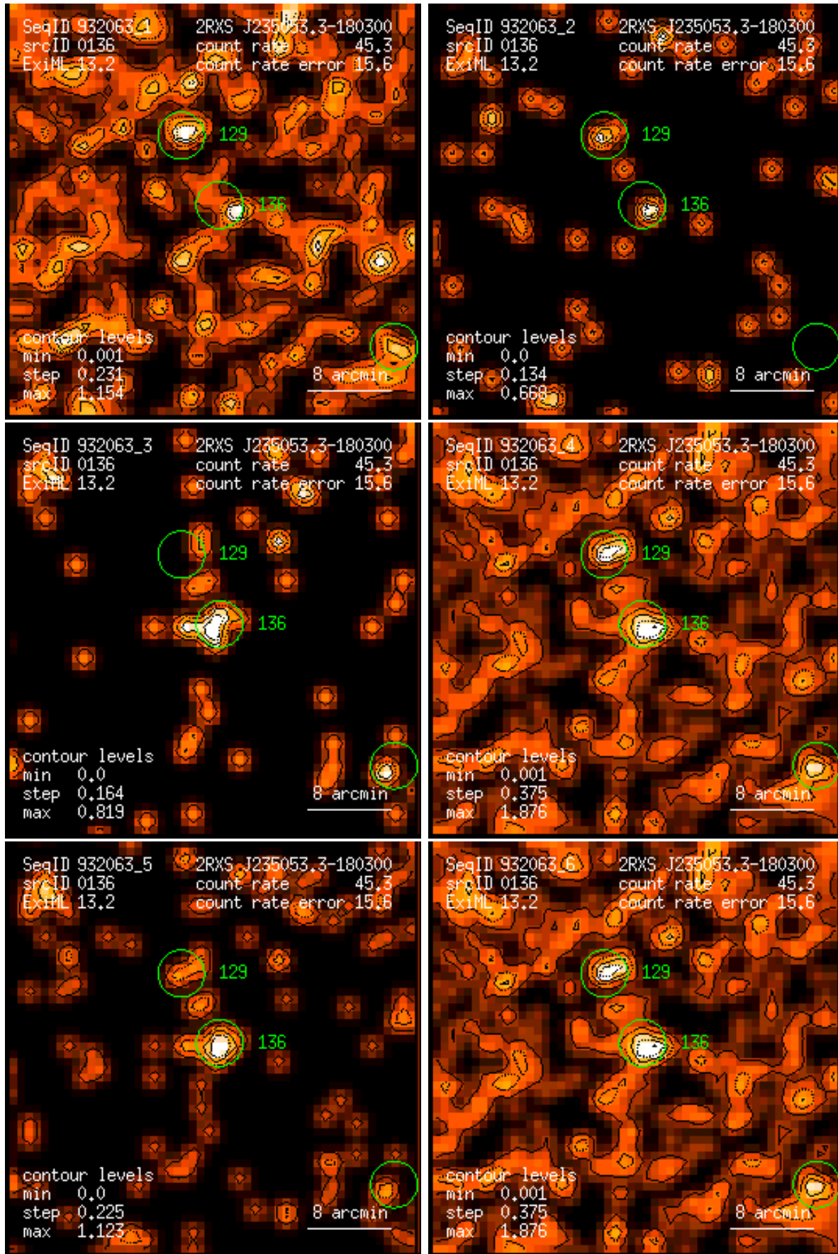
Figure 136: RASS 932063: detection 0136: band rate images, Gaussian filter: (1) PSPC channels 11 – 41, (2) 52 – 90, (3) 91 – 201, (4) 11 – 235, (5) 52 – 201, (6) 11 – 201. Broad band rates in counts/ks. Band rate contour levels in counts/ks/arcmin 2 .
