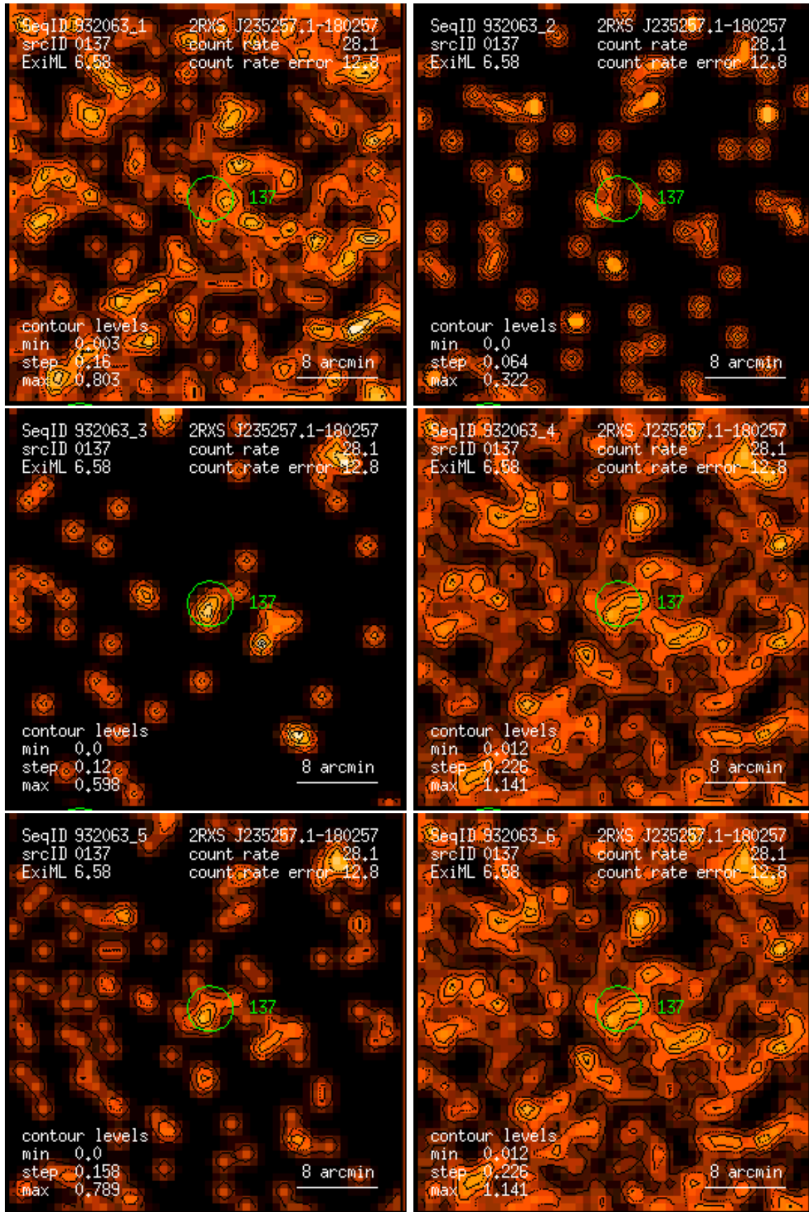
Figure 137: RASS 932063: detection 0137: band rate images, Gaussian filter: (1) PSPC channels 11 – 41, (2) 52 – 90, (3) 91 – 201, (4) 11 – 235, (5) 52 – 201, (6) 11 – 201. Broad band rates in counts/ks. Band rate contour levels in counts/ks/arcmin 2 .
