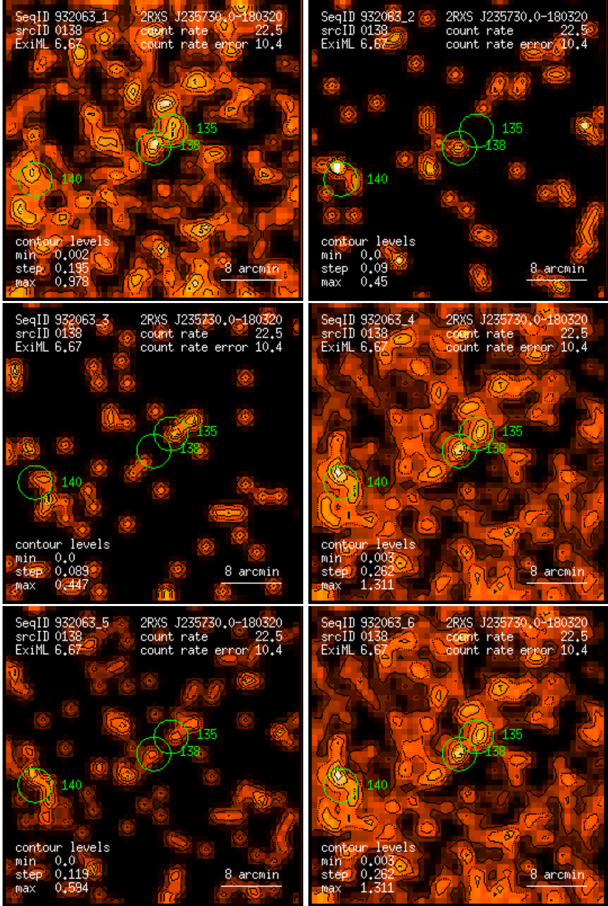
Figure 138: RASS 932063: detection 0138: band rate images, Gaussian filter: (1) PSPPC channels 11 – 41, (2) 52 – 90, (3) 91 – 201, (4) 11 – 235, (5) 52 – 201, (6) 11 – 201. Broad band rates in counts/ks. Band rate contour levels in counts/ks/arcmin 2 .
