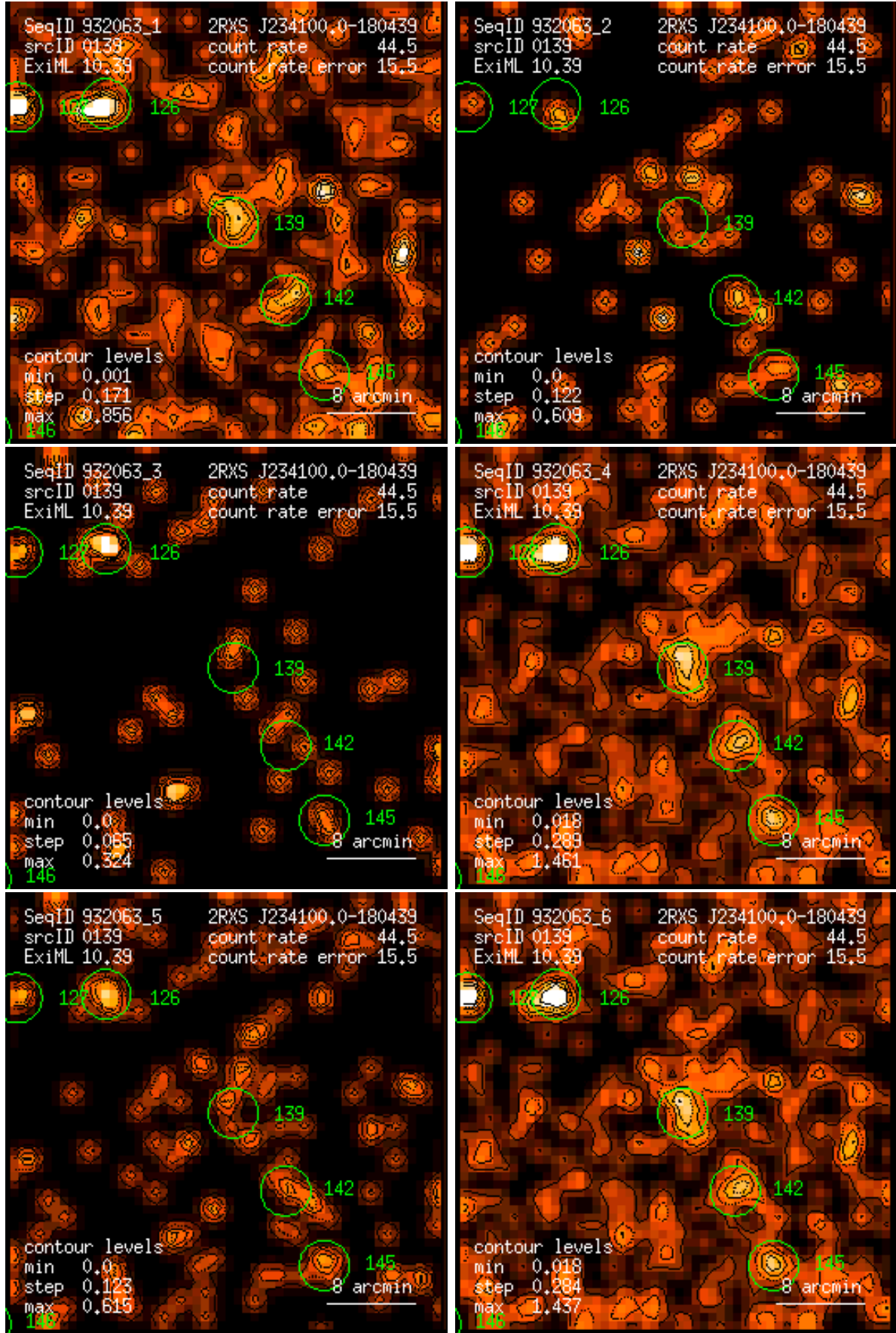
Figure 139: RASS 932063: detection 0139: band rate images, Gaussian filter: (1) PSPC channels 11 – 41, (2) 52 – 90, (3) 91 – 201, (4) 11 – 235, (5) 52 – 201, (6) 11 – 201. Broad band rates in counts/ks. Band rate contour levels in counts/ks/arcmin 2 .
