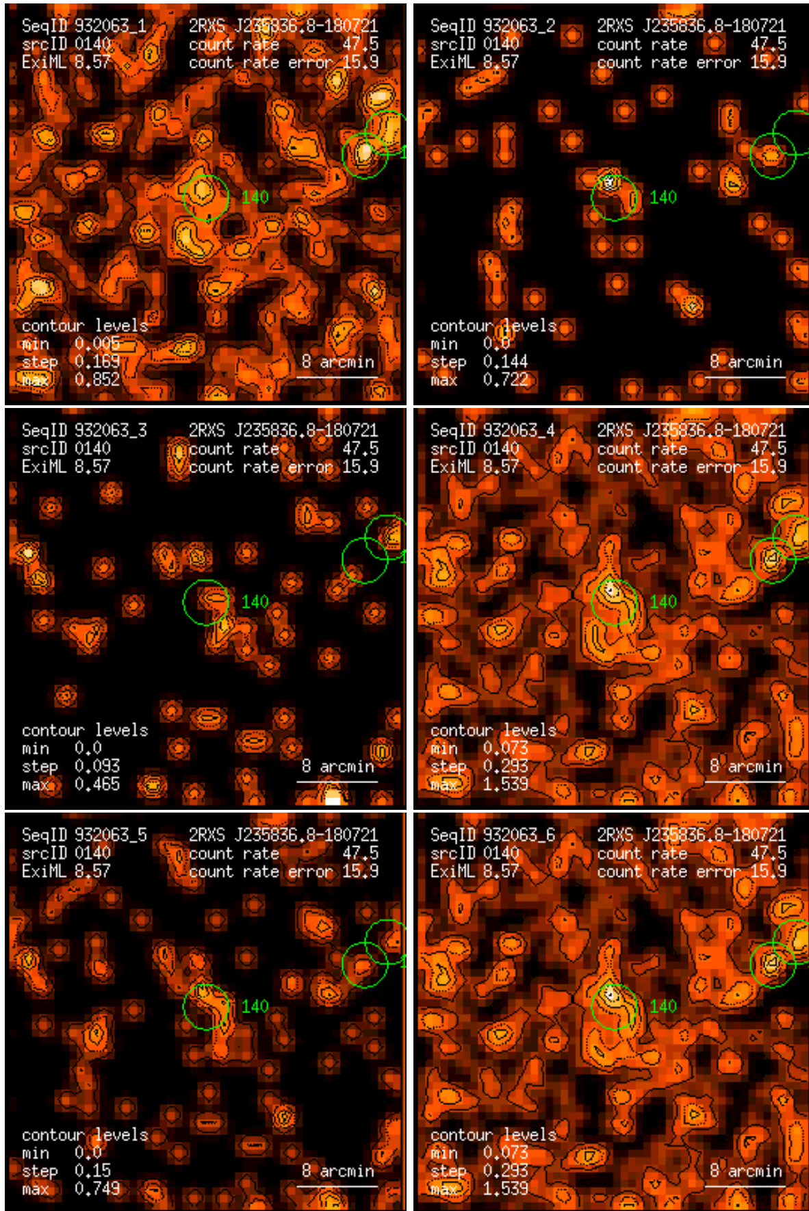
Figure 140: RASS 932063: detection 0140: band rate images, Gaussian filter: (1) PSPC channels 11 – 41, (2) 52 – 90, (3) 91 – 201, (4) 11 – 235, (5) 52 – 201, (6) 11 – 201. Broad band rates in counts/ks. Band rate contour levels in counts/ks/arcmin 2 .
