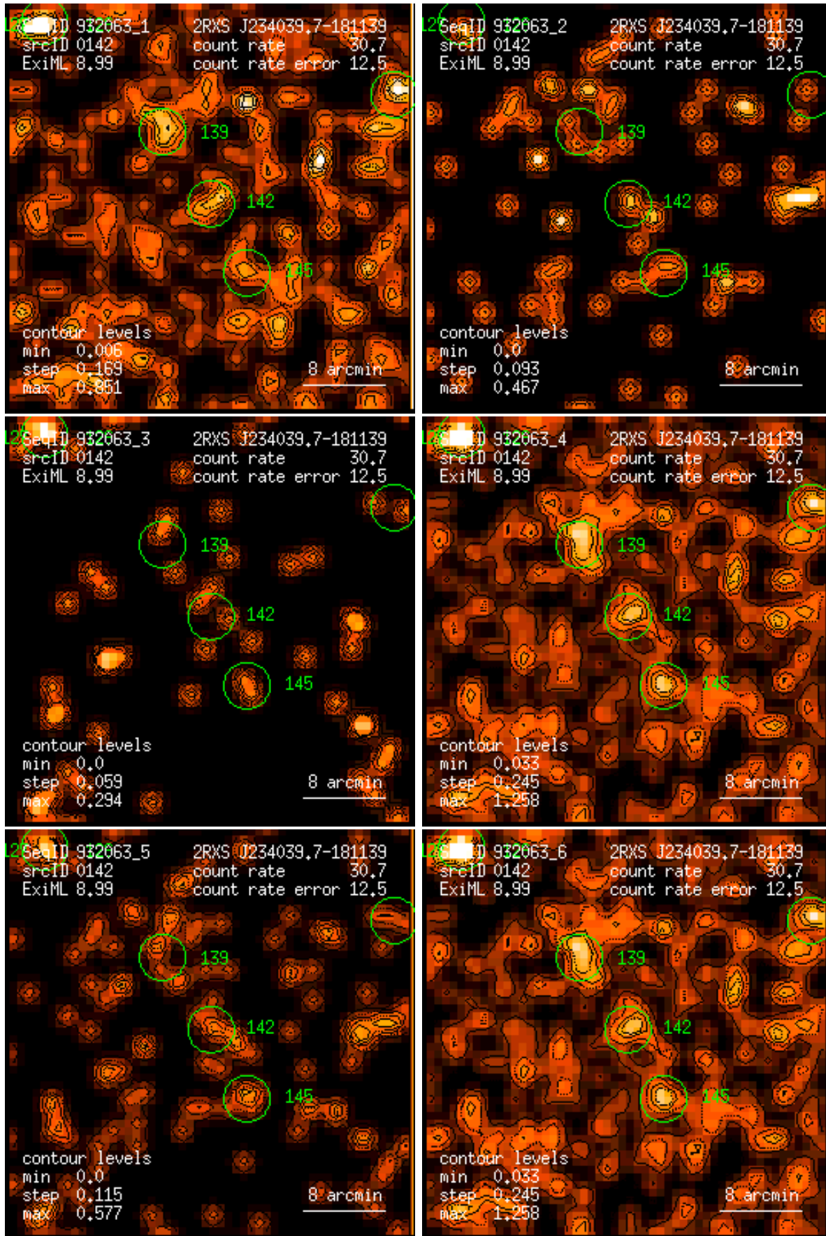
Figure 142: RASS 932063: detection 0142: band rate images, Gaussian filter: (1) PSPC channels 11 – 41, (2) 52 – 90, (3) 91 – 201, (4) 11 – 235, (5) 52 – 201, (6) 11 – 201. Broad band rates in counts/ks. Band rate contour levels in counts/ks/arcmin 2 .
