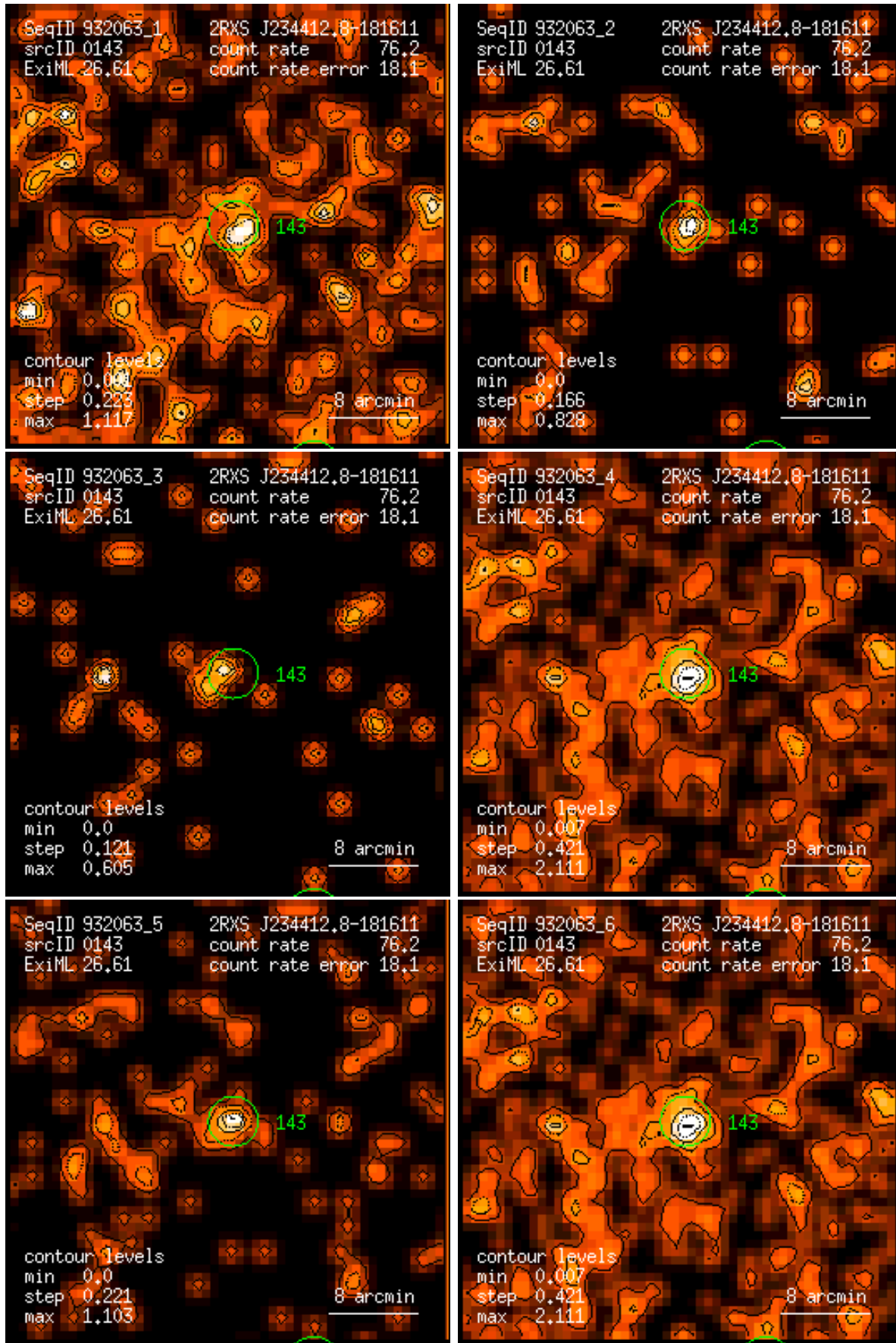
Figure 143: RASS 932063: detection 0143: band rate images, Gaussian filter: (1) PSPC channels 11 – 41, (2) 52 – 90, (3) 91 – 201, (4) 11 – 235, (5) 52 – 201, (6) 11 – 201. Broad band rates in counts/ks. Band rate contour levels in counts/ks/arcmin 2 .
