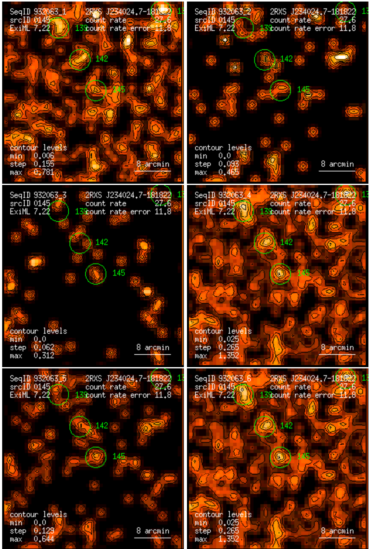
Figure 145: RASS 932063: detection 0145: band rate images, Gaussian filter: (1) PSPC channels 11 – 41, (2) 52 – 90, (3) 91 – 201, (4) 11 – 235, (5) 52 – 201, (6) 11 – 201. Broad band rates in counts/ks. Band rate contour levels in counts/ks/arcmin 2 .
