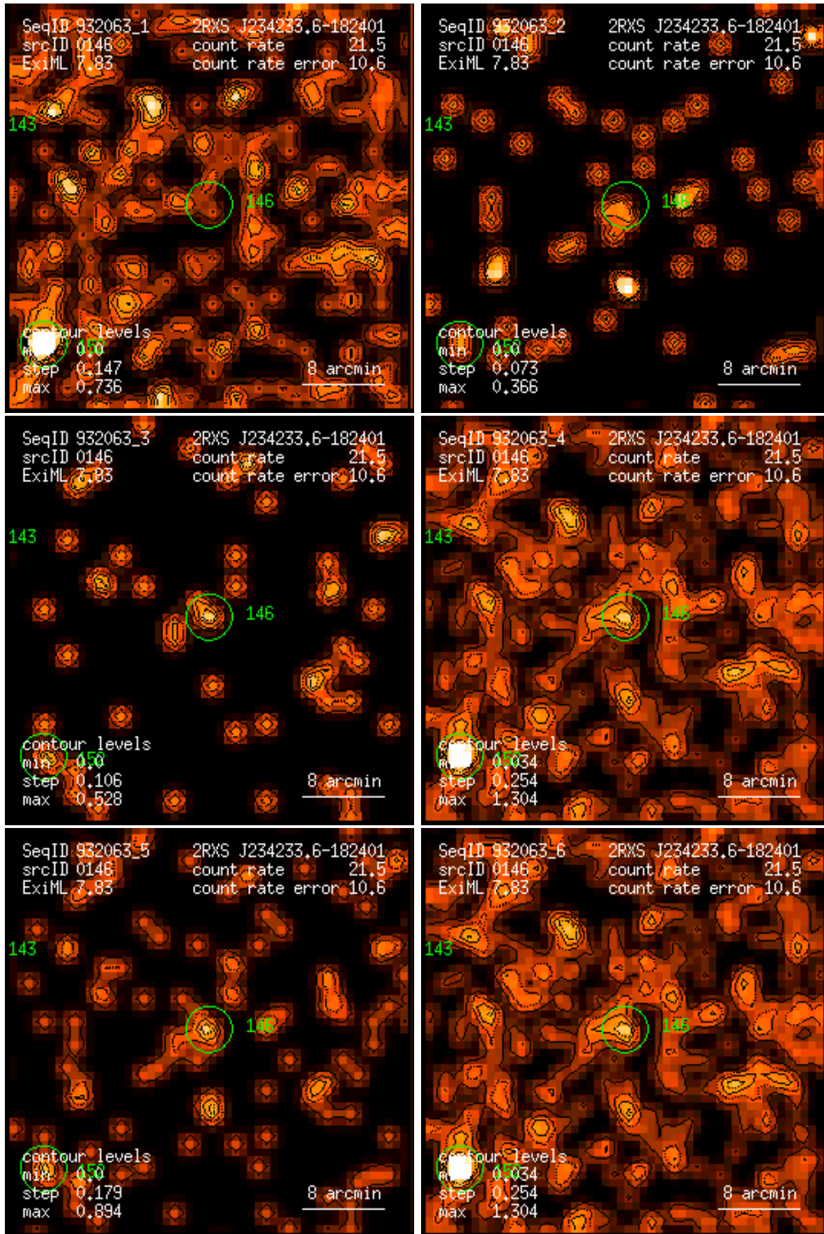
Figure 146: RASS 932063: detection 0146: band rate images, Gaussian filter: (1) PSPC channels 11 – 41, (2) 52 – 90, (3) 91 – 201, (4) 11 – 235, (5) 52 – 201, (6) 11 – 201. Broad band rates in counts/ks. Band rate contour levels in counts/ks/arcmin 2 .
