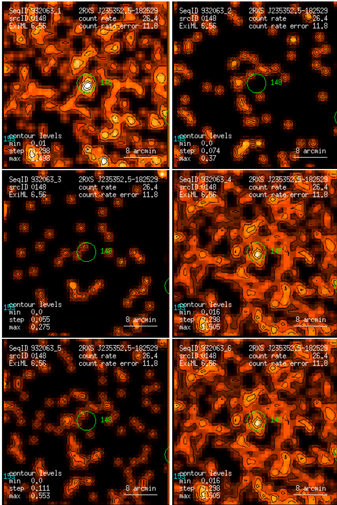
Figure 148: RASS 932063: detection 0148: band rate images, Gaussian filter: (1) PSPC channels 11 – 41, (2) 52 – 90, (3) 91 – 201, (4) 11 – 235, (5) 52 – 201, (6) 11 – 201. Broad band rates in counts/ks. Band rate contour levels in counts/ks/arcmin 2 .
