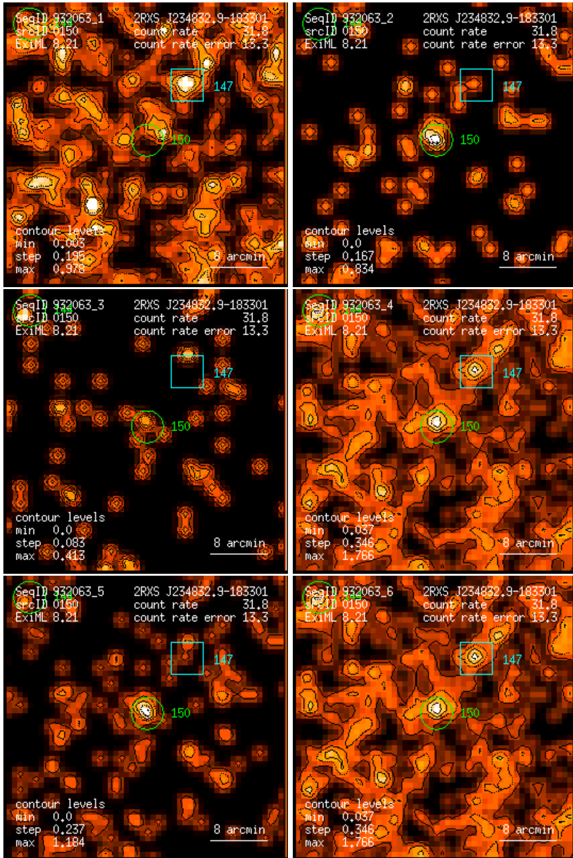
Figure 150: RASS 932063: detection 0150: band rate images, Gaussian filter: (1) PSPC channels 11 – 41, (2) 52 – 90, (3) 91 – 201, (4) 11 – 235, (5) 52 – 201, (6) 11 – 201. Broad band rates in counts/ks. Band rate contour levels in counts/ks/arcmin 2 .
