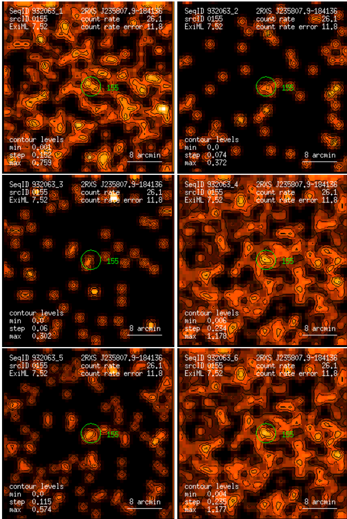
Figure 155: RASS 932063: detection 0155: band rate images, Gaussian filter: (1) PSPC channels 11 – 41, (2) 52 – 90, (3) 91 – 201, (4) 11 – 235, (5) 52 – 201, (6) 11 – 201. Broad band rates in counts/ks. Band rate contour levels in counts/ks/arcmin 2 .
