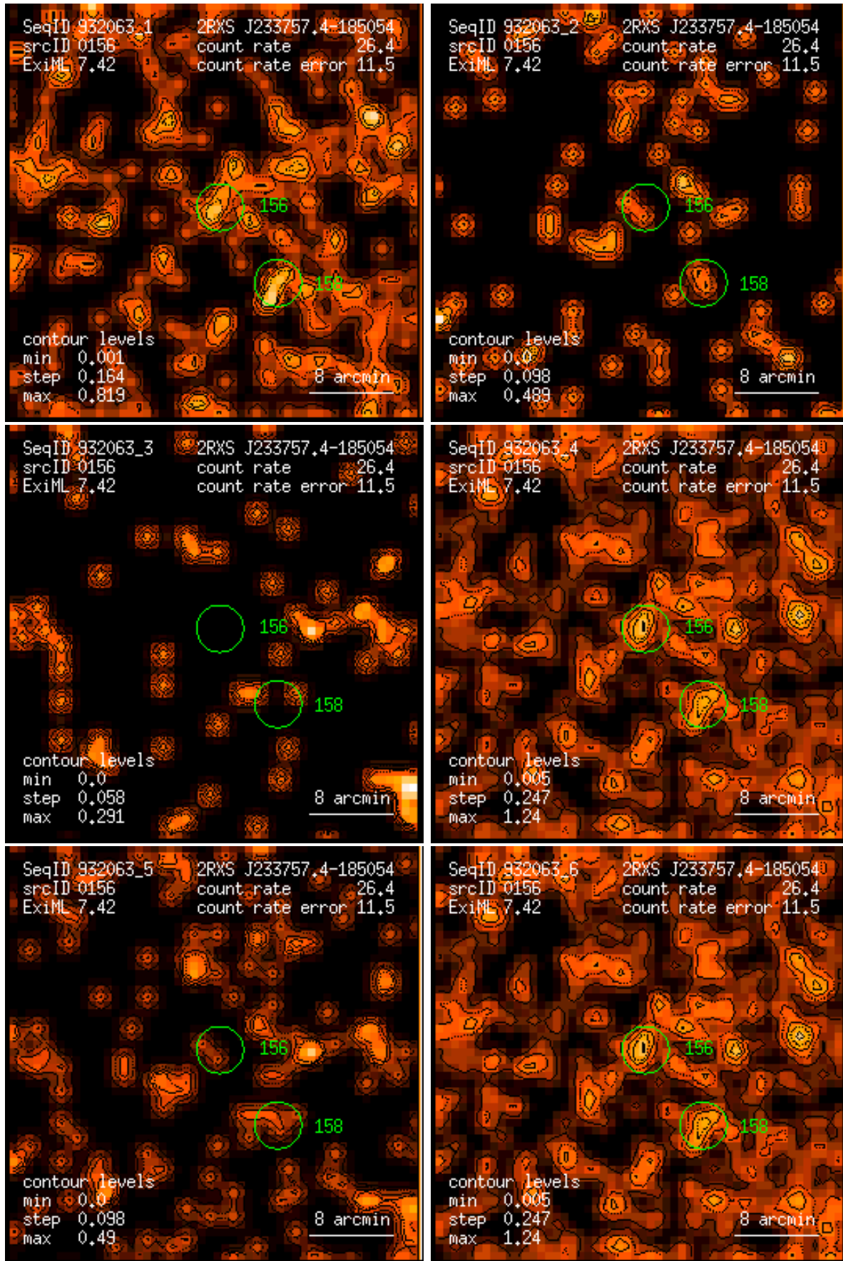
Figure 156: RASS 932063: detection 0156: band rate images, Gaussian filter: (1) PSPC channels 11 – 41, (2) 52 – 90, (3) 91 – 201, (4) 11 – 235, (5) 52 – 201, (6) 11 – 201. Broad band rates in counts/ks. Band rate contour levels in counts/ks/arcmin 2 .
