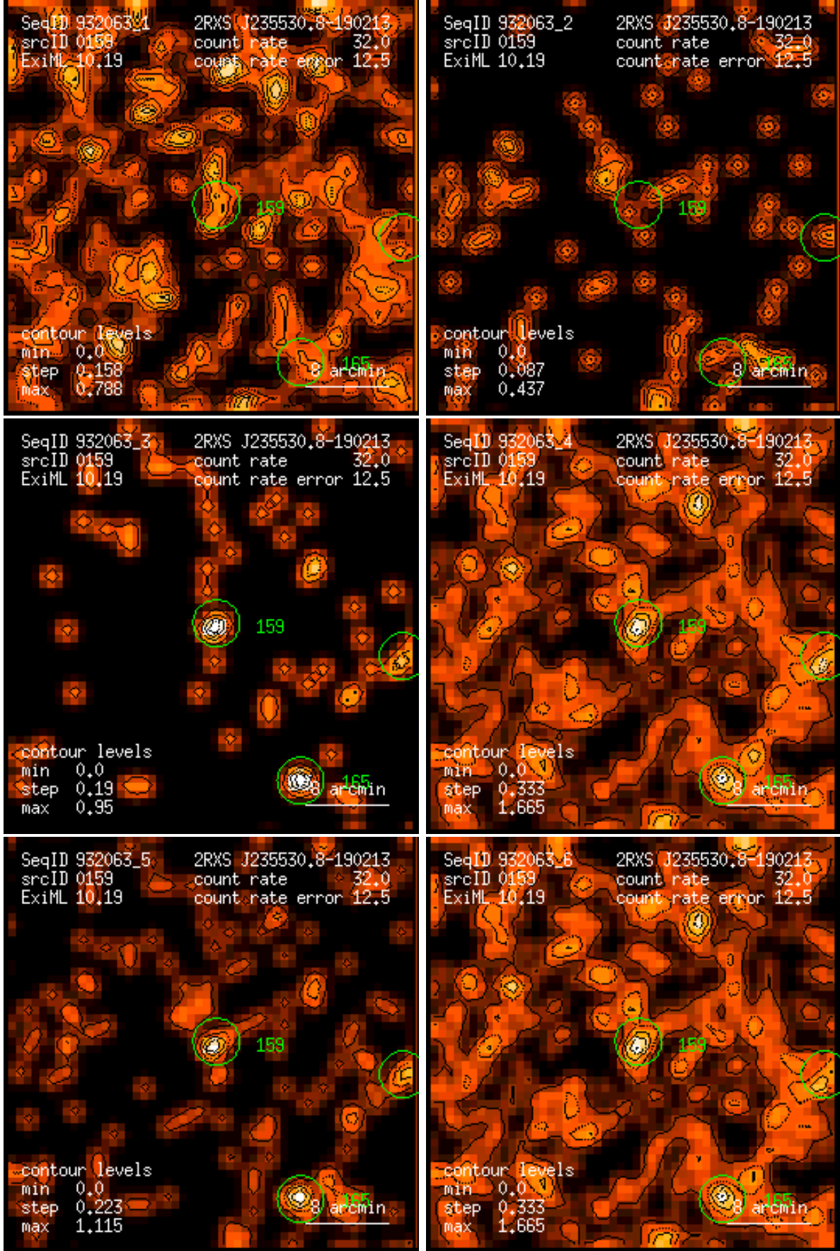
Figure 159: RASS 932063: detection 0159: band rate images, Gaussian filter: (1) PSPC channels 11 – 41, (2) 52 – 90, (3) 91 – 201, (4) 11 – 235, (5) 52 – 201, (6) 11 – 201. Broad band rates in counts/ks. Band rate contour levels in counts/ks/arcmin 2 .
