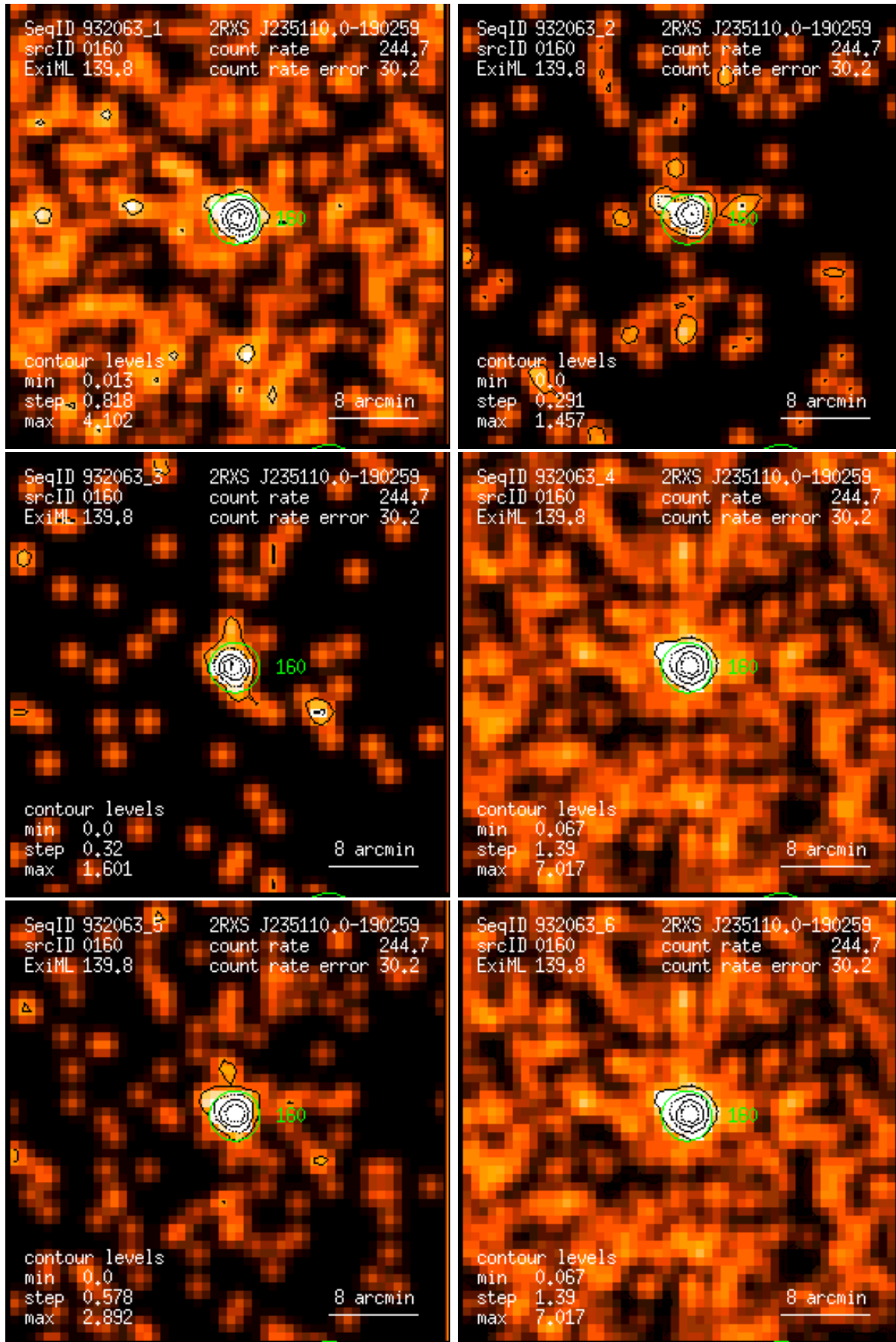
Figure 160: RASS 932063: detection 0160: band rate images, Gaussian filter: (1) PSPC channels 11 – 41, (2) 52 – 90, (3) 91 – 201, (4) 11 – 235, (5) 52 – 201, (6) 11 – 201. Broad band rates in counts/ks. Band rate contour levels in counts/ks/arcmin 2 .
