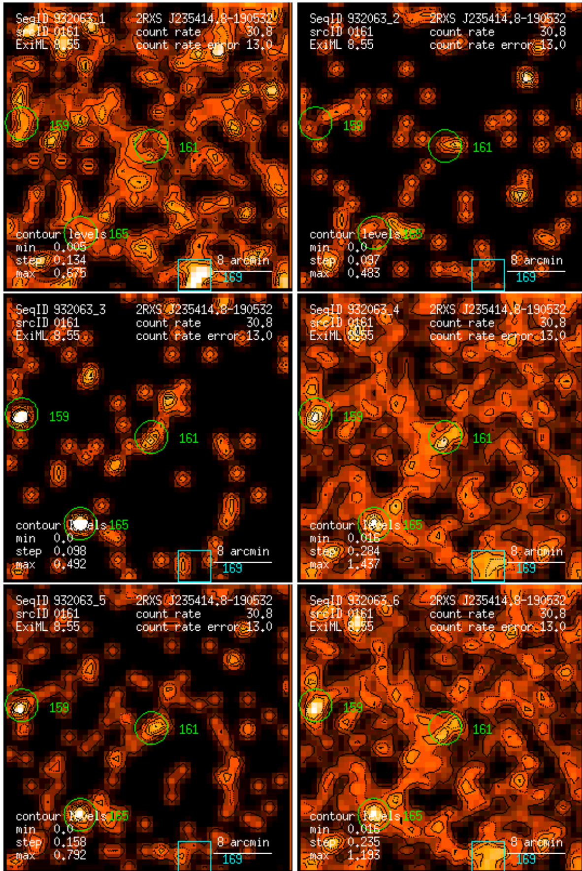
Figure 161: RASS 932063: detection 0161: band rate images, Gaussian filter: (1) PSPC channels 11 – 41, (2) 52 – 90, (3) 91 – 201, (4) 11 – 235, (5) 52 – 201, (6) 11 – 201. Broad band rates in counts/ks. Band rate contour levels in counts/ks/arcmin 2 .
