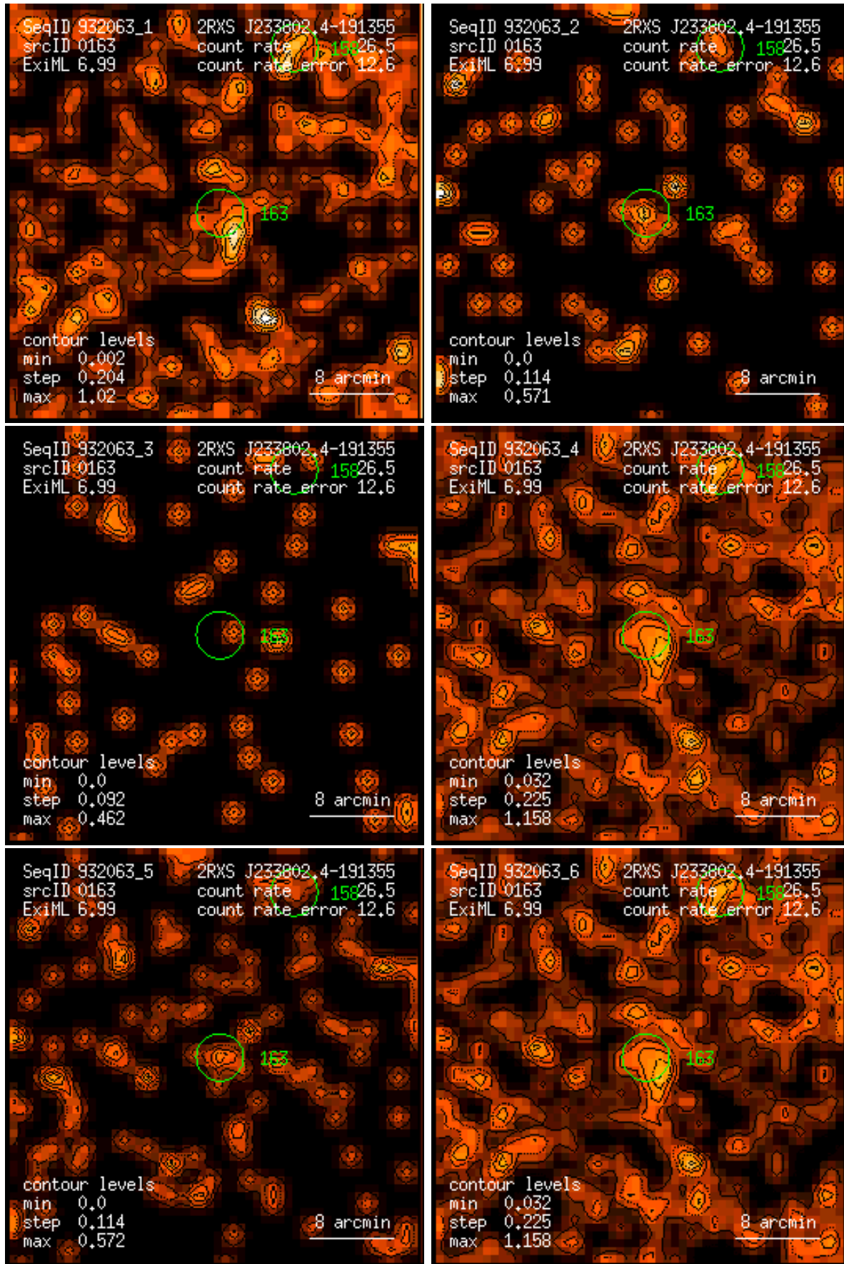
Figure 163: RASS 932063: detection 0163: band rate images, Gaussian filter: (1) PSPC channels 11 – 41, (2) 52 – 90, (3) 91 – 201, (4) 11 – 235, (5) 52 – 201, (6) 11 – 201. Broad band rates in counts/ks. Band rate contour levels in counts/ks/arcmin 2 .
