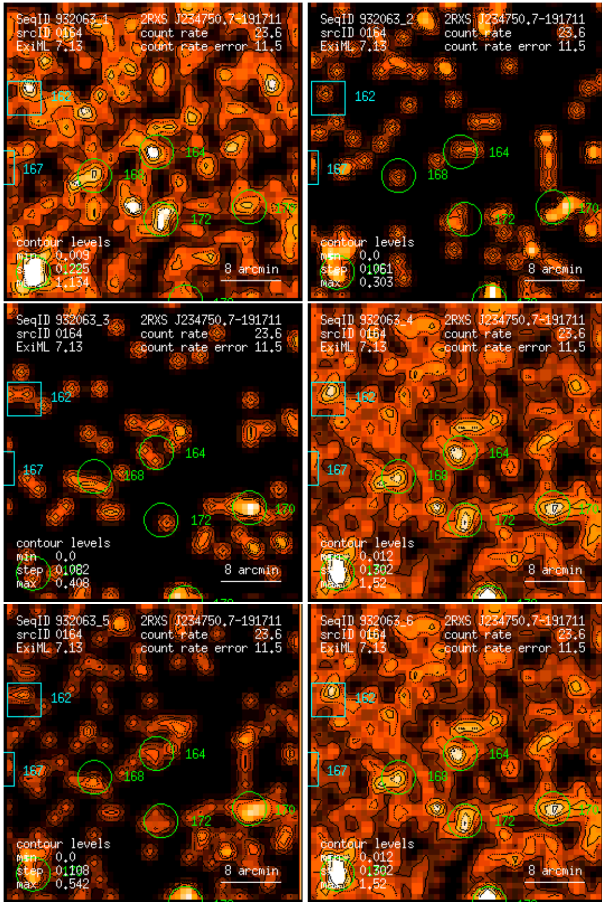
Figure 164: RASS 932063: detection 0164: band rate images, Gaussian filter: (1) PSPC channels 11 – 41, (2) 52 – 90, (3) 91 – 201, (4) 11 – 235, (5) 52 – 201, (6) 11 – 201. Broad band rates in counts/ks. Band rate contour levels in counts/ks/arcmin 2 .
