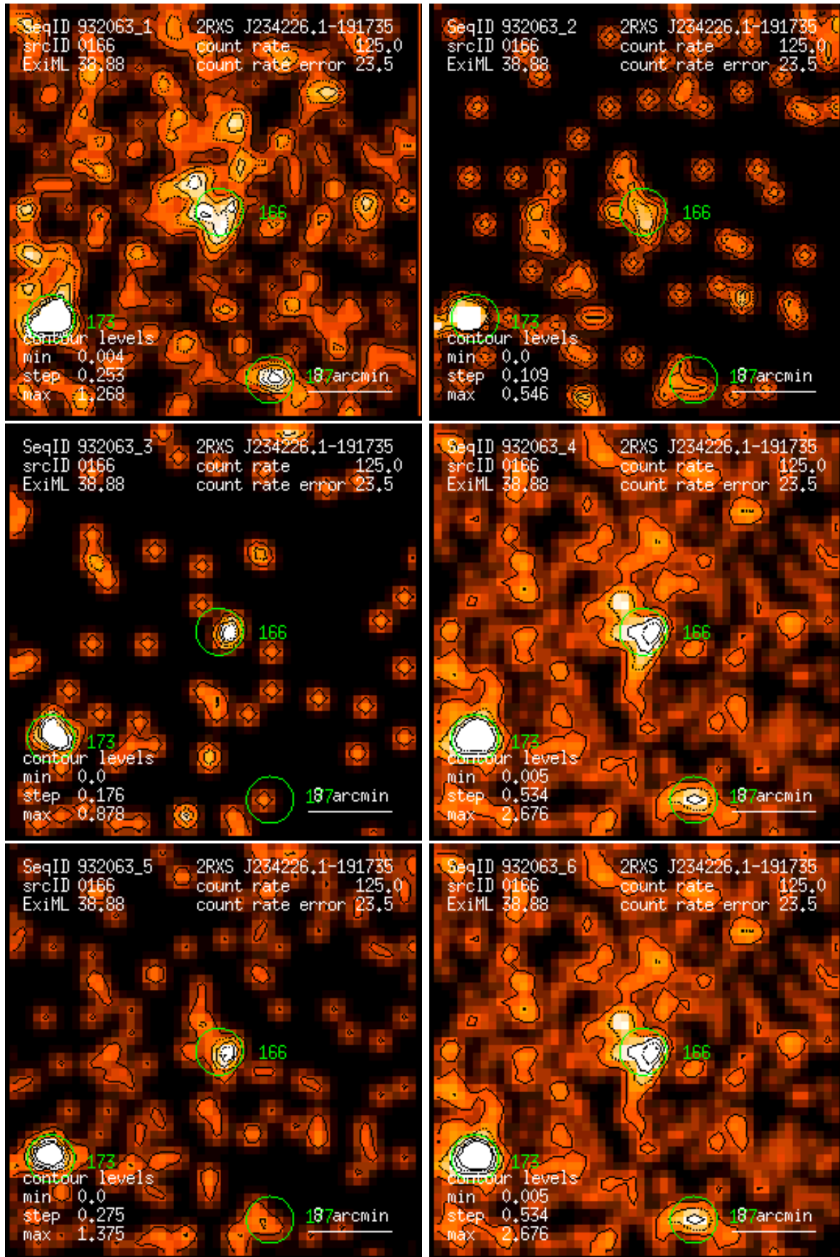
Figure 166: RASS 932063: detection 0166: band rate images, Gaussian filter: (1) PSPC channels 11 – 41, (2) 52 – 90, (3) 91 – 201, (4) 11 – 235, (5) 52 – 201, (6) 11 – 201. Broad band rates in counts/ks. Band rate contour levels in counts/ks/arcmin 2 .
