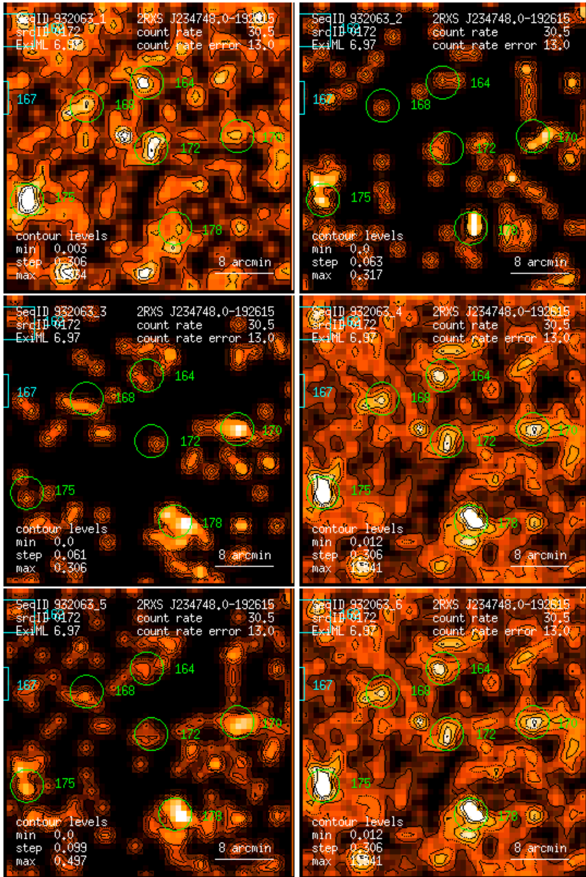
Figure 172: RASS 932063: detection 0172: band rate images, Gaussian filter: (1) PSPC channels 11 – 41, (2) 52 – 90, (3) 91 – 201, (4) 11 – 235, (5) 52 – 201, (6) 11 – 201. Broad band rates in counts/ks. Band rate contour levels in counts/ks/arcmin 2 .
