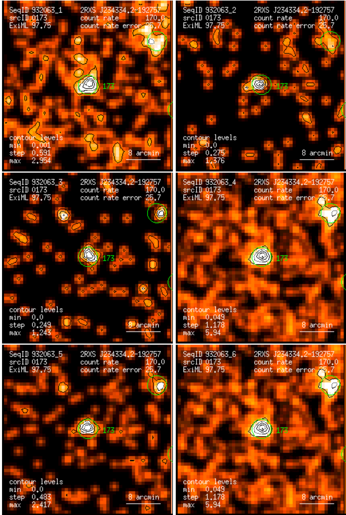
Figure 173: RASS 932063: detection 0173: band rate images, Gaussian filter: (1) PSPC channels 11 – 41, (2) 52 – 90, (3) 91 – 201, (4) 11 – 235, (5) 52 – 201, (6) 11 – 201. Broad band rates in counts/ks. Band rate contour levels in counts/ks/arcmin 2 .
