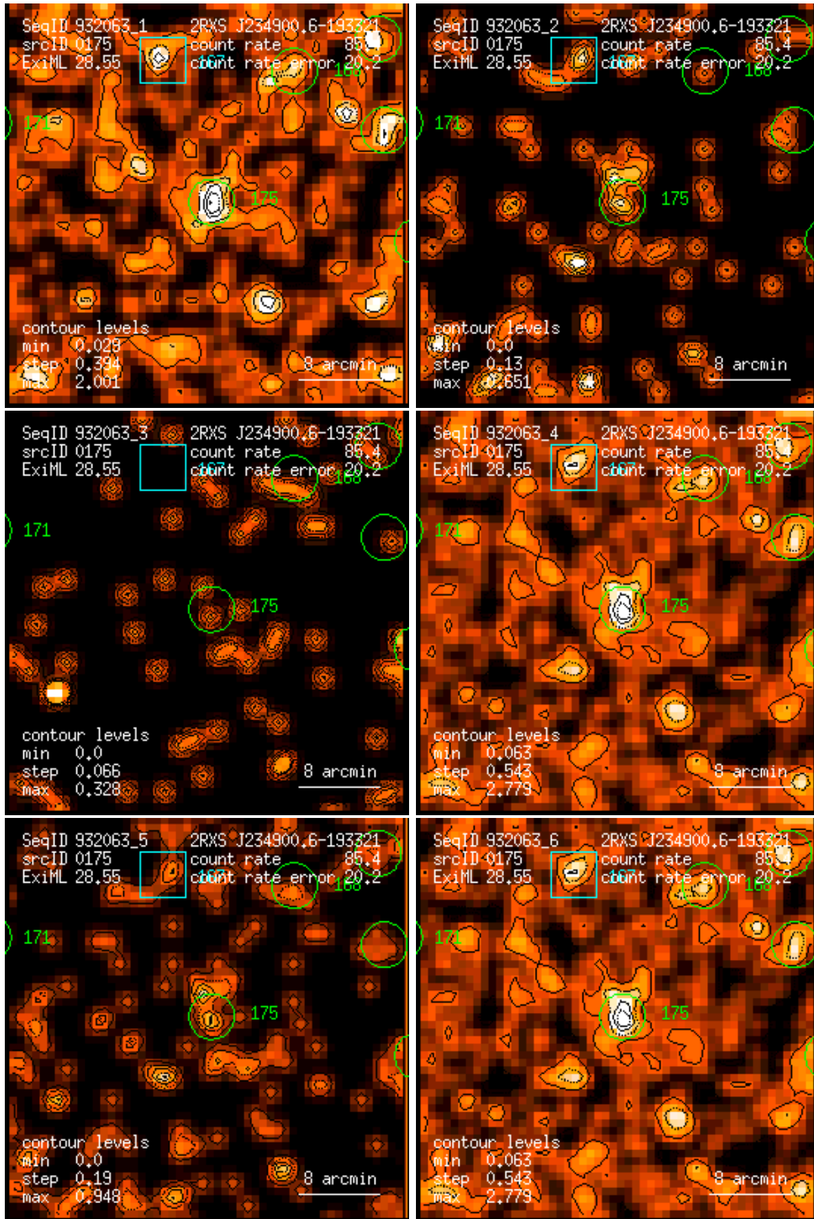
Figure 175: RASS 932063: detection 0175: band rate images, Gaussian filter: (1) PSPC channels 11 – 41, (2) 52 – 90, (3) 91 – 201, (4) 11 – 235, (5) 52 – 201, (6) 11 – 201. Broad band rates in counts/ks. Band rate contour levels in counts/ks/arcmin 2 .
