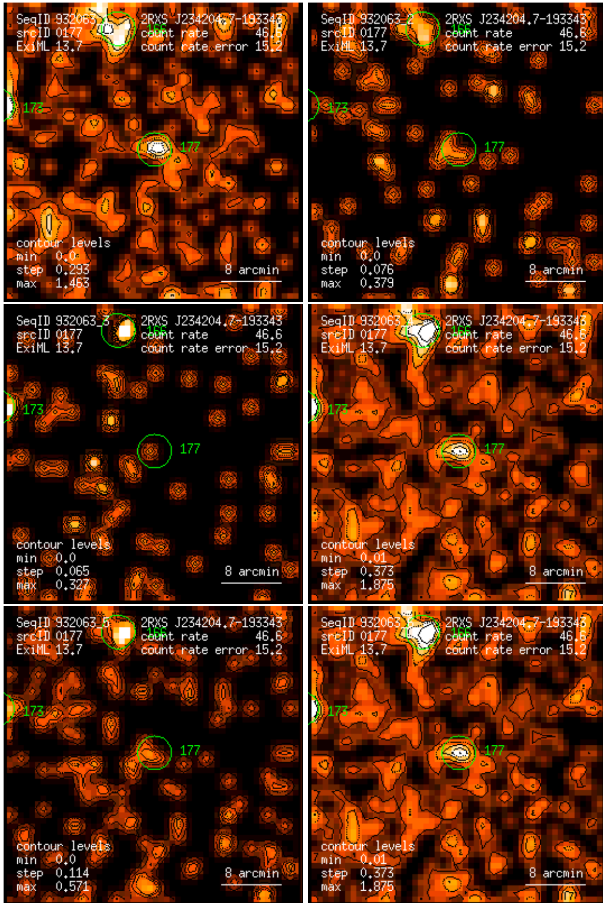
Figure 177: RASS 932063: detection 0177: band rate images, Gaussian filter: (1) PSPC channels 11 – 41, (2) 52 – 90, (3) 91 – 201, (4) 11 – 235, (5) 52 – 201, (6) 11 – 201. Broad band rates in counts/ks. Band rate contour levels in counts/ks/arcmin 2 .
