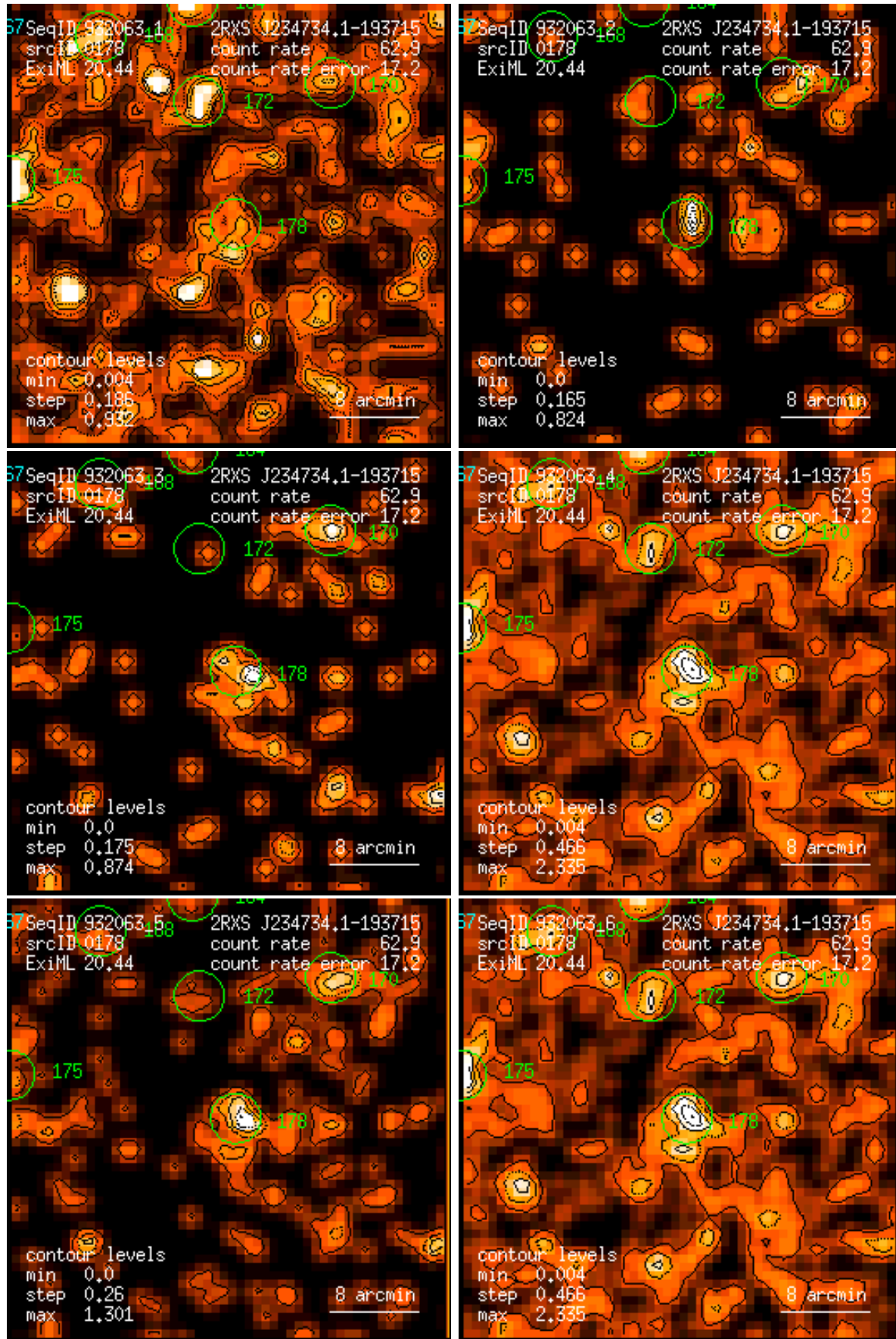
Figure 178: RASS 932063: detection 0178: band rate images, Gaussian filter: (1) PSPC channels 11 – 41, (2) 52 – 90, (3) 91 – 201, (4) 11 – 235, (5) 52 – 201, (6) 11 – 201. Broad band rates in counts/ks. Band rate contour levels in counts/ks/arcmin 2 .
