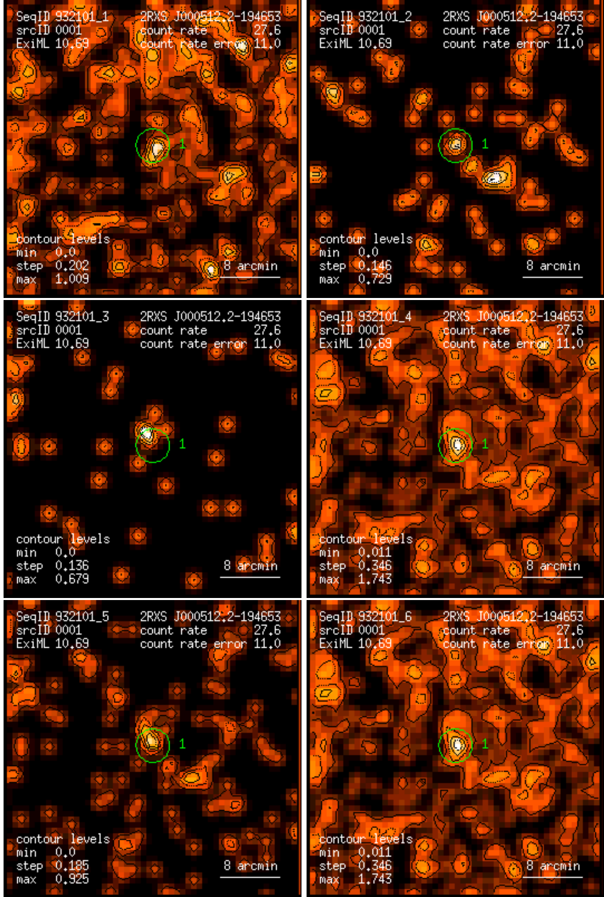
Figure 1: RASS 932101: detection 0001: band rate images, Gaussian filter: (1) PSPC channels 11 – 41, (2) 52 – 90, (3) 91 – 201, (4) 11 – 235, (5) 52 – 201, (6) 11 – 201. Broad band rates in counts/ks. Band rate contour levels in counts/ks/arcmin 2 .
