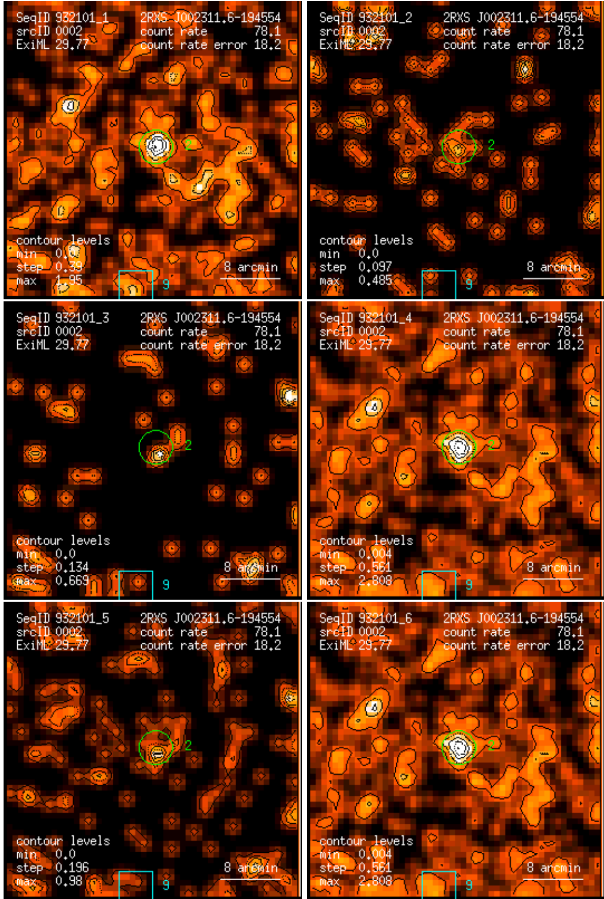
Figure 2: RASS 932101: detection 0002: band rate images, Gaussian filter: (1) PSPC channels 11 – 41, (2) 52 – 90, (3) 91 – 201, (4) 11 – 235, (5) 52 – 201, (6) 11 – 201. Broad band rates in counts/ks. Band rate contour levels in counts/ks/arcmin 2 .
