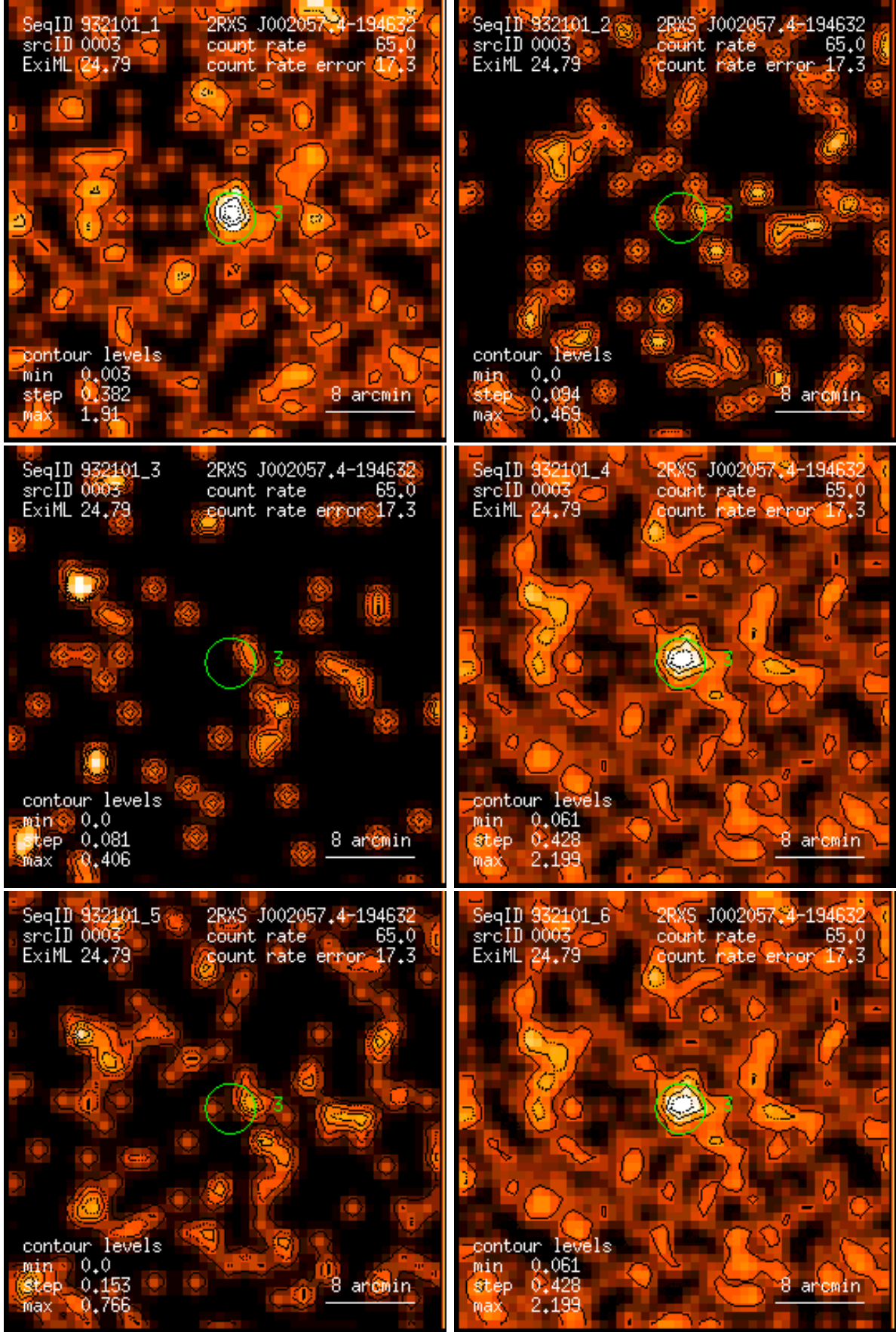
Figure 3: RASS 932101: detection 0003: band rate images, Gaussian filter: (1) PSPC channels 11 – 41, (2) 52 – 90, (3) 91 – 201, (4) 11 – 235, (5) 52 – 201, (6) 11 – 201. Broad band rates in counts/ks. Band rate contour levels in counts/ks/arcmin 2 .
