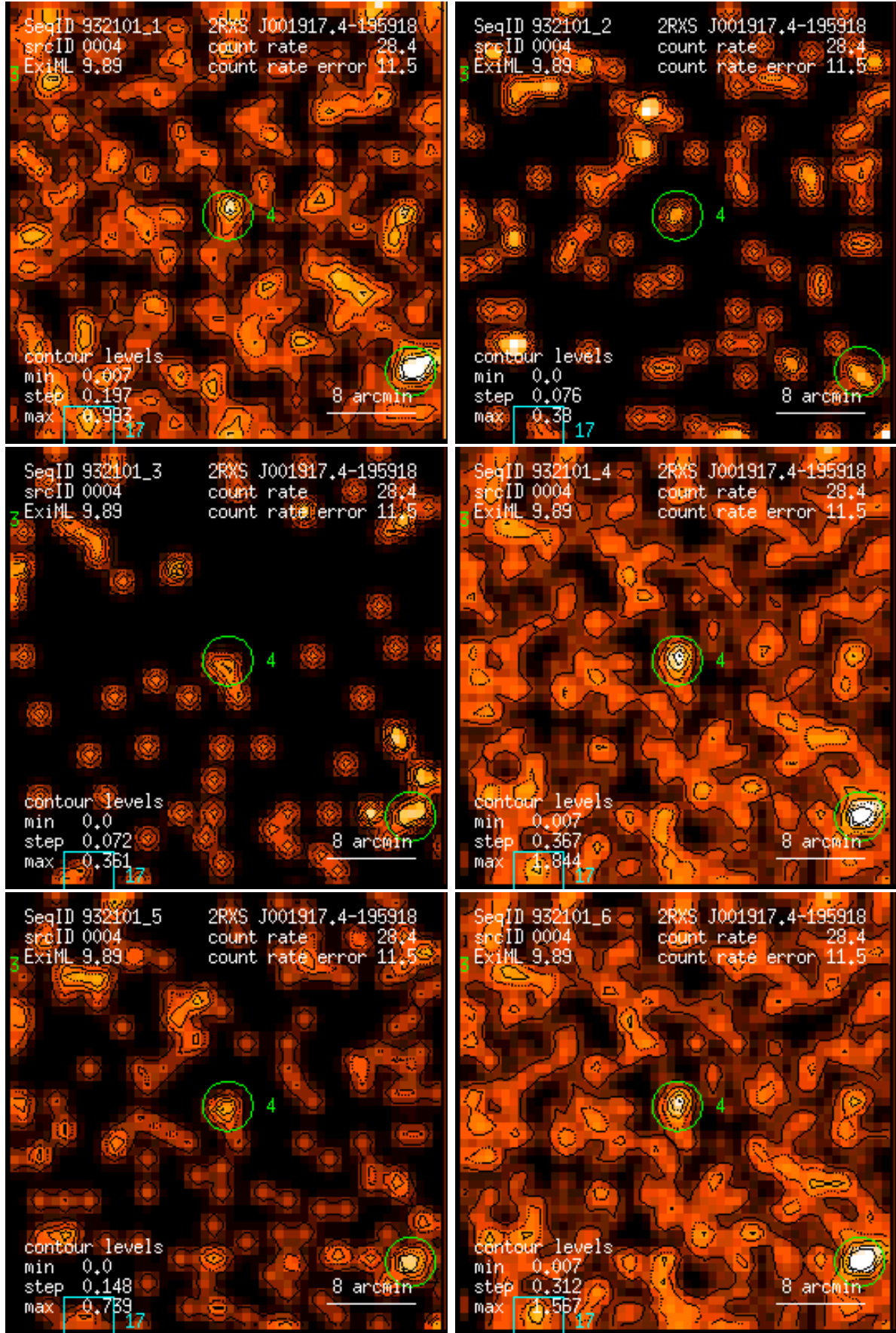
Figure 4: RASS 932101: detection 0004: band rate images, Gaussian filter: (1) PSPC channels 11 – 41, (2) 52 – 90, (3) 91 – 201, (4) 11 – 235, (5) 52 – 201, (6) 11 – 201. Broad band rates in counts/ks. Band rate contour levels in counts/ks/arcmin 2 .
