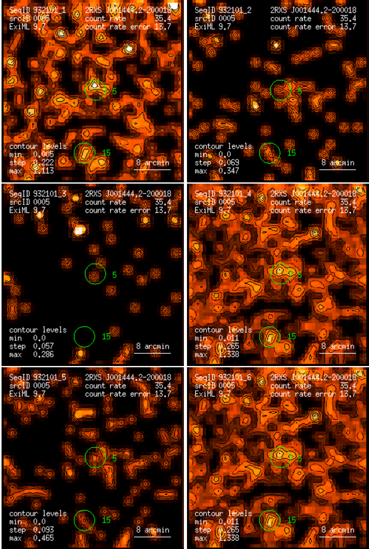
Figure 5: RASS 932101: detection 0005: band rate images, Gaussian filter: (1) PSPC channels 11 – 41, (2) 52 – 90, (3) 91 – 201, (4) 11 – 235, (5) 52 – 201, (6) 11 – 201. Broad band rates in counts/ks. Band rate contour levels in counts/ks/arcmin 2 .
