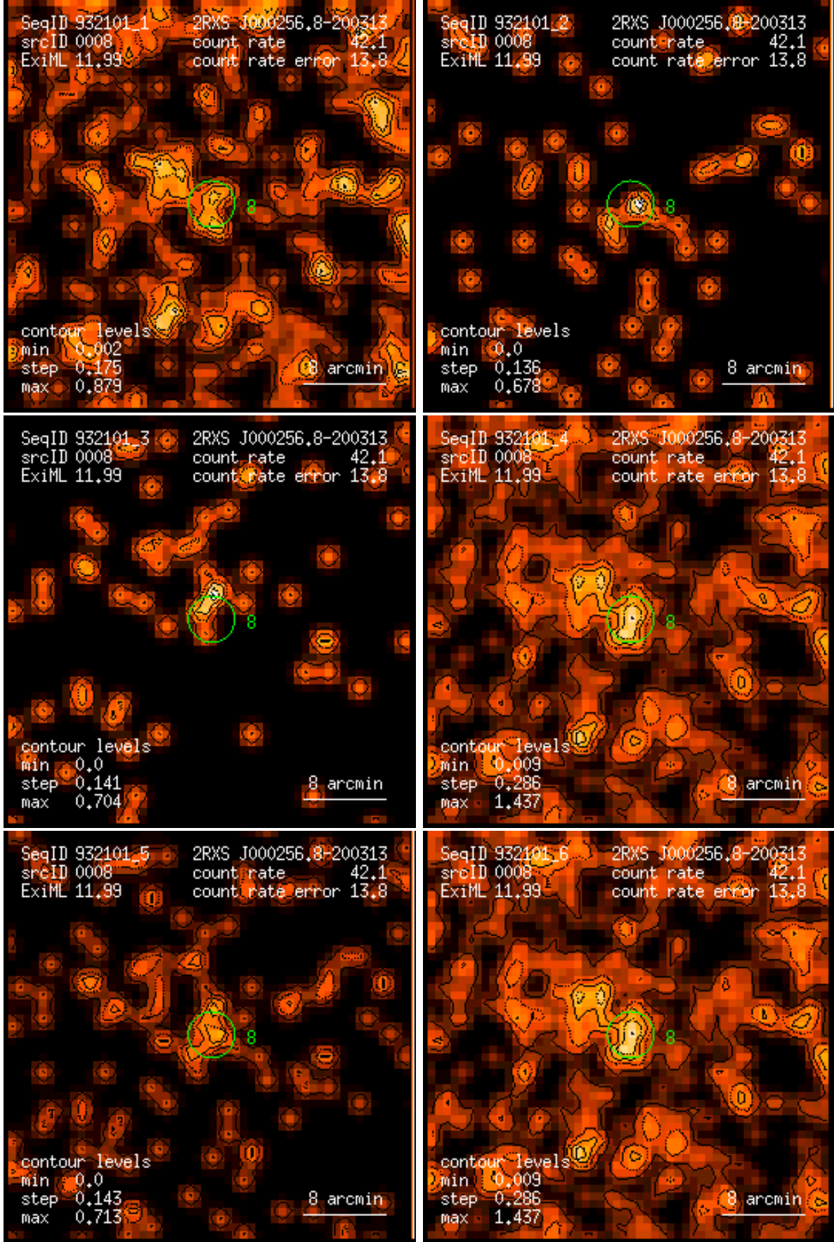
Figure 8: RASS 932101: detection 0008: band rate images, Gaussian filter: (1) PSPC channels 11 – 41, (2) 52 – 90, (3) 91 – 201, (4) 11 – 235, (5) 52 – 201, (6) 11 – 201. Broad band rates in counts/ks. Band rate contour levels in counts/ks/arcmin 2 .
