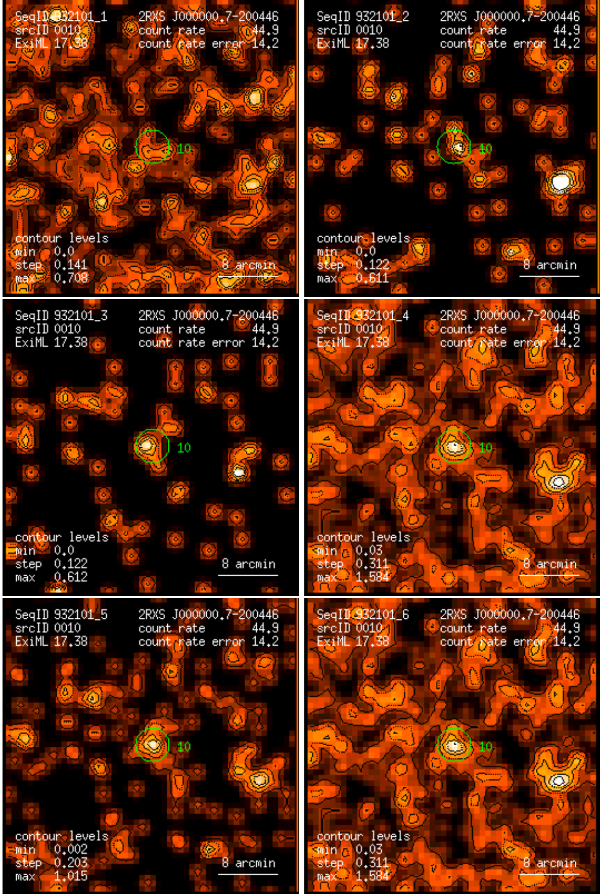
Figure 10: RASS 932101: detection 0010: band rate images, Gaussian filter: (1) PSPC channels 11 – 41, (2) 52 – 90, (3) 91 – 201, (4) 11 – 235, (5) 52 – 201, (6) 11 – 201. Broad band rates in counts/ks. Band rate contour levels in counts/ks/arcmin 2 .
