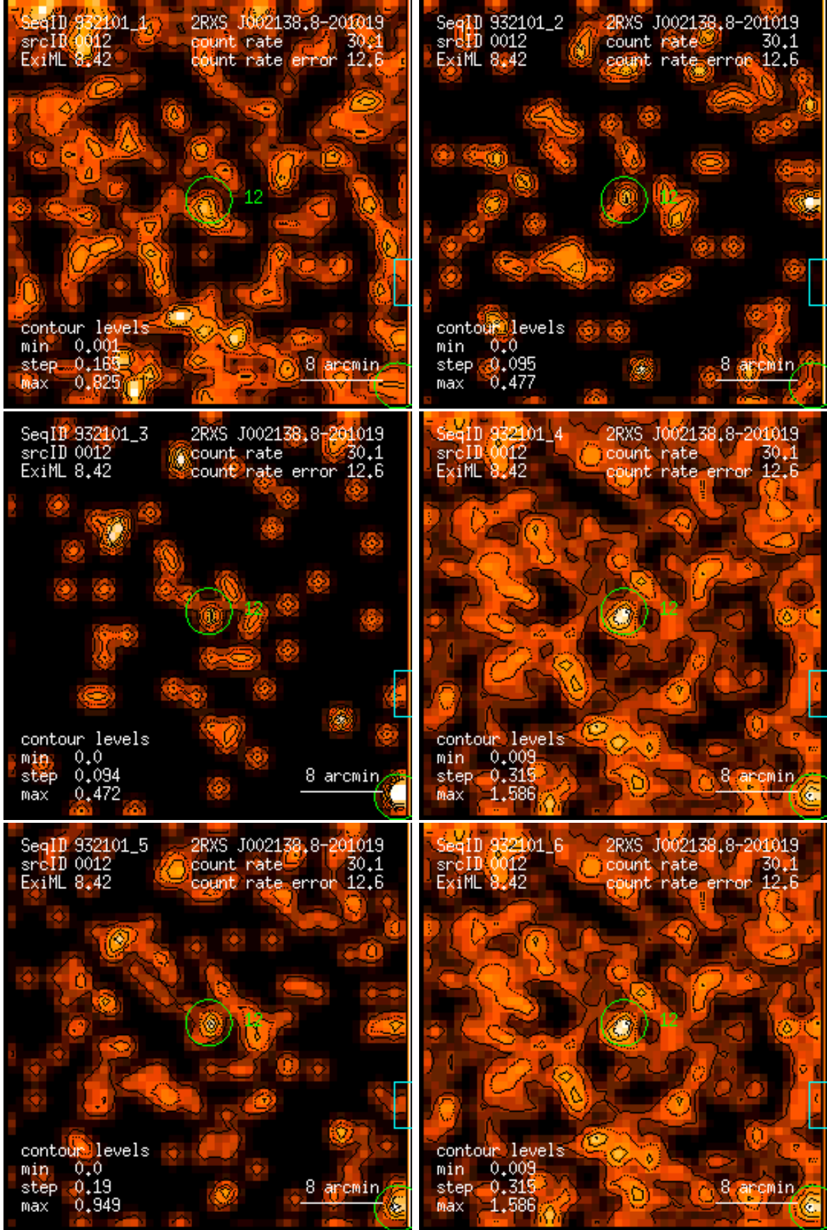
Figure 12: RASS 932101: detection 0012: band rate images, Gaussian filter: (1) PSPC channels 11 – 41, (2) 52 – 90, (3) 91 – 201, (4) 11 – 235, (5) 52 – 201, (6) 11 – 201. Broad band rates in counts/ks. Band rate contour levels in counts/ks/arcmin 2 .
