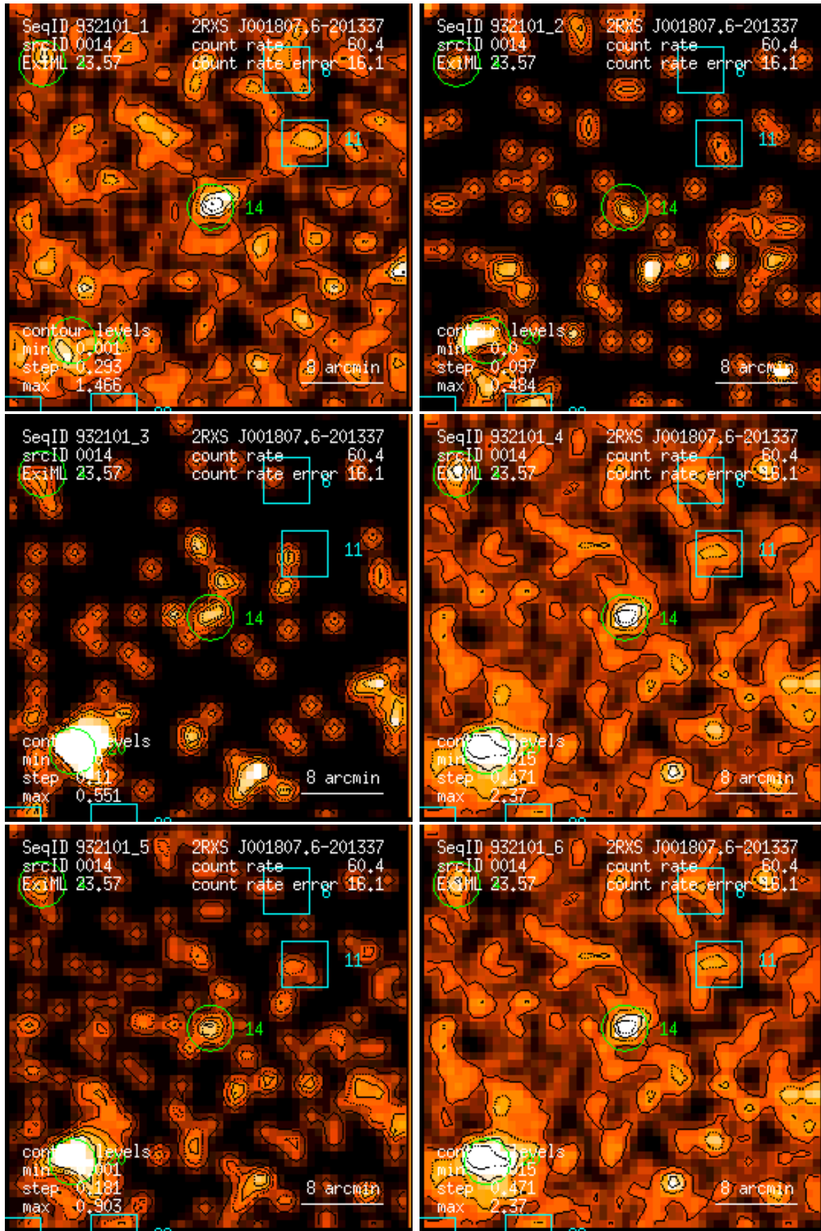
Figure 14: RASS 932101: detection 0014: band rate images, Gaussian filter: (1) PSPC channels 11 – 41, (2) 52 – 90, (3) 91 – 201, (4) 11 – 235, (5) 52 – 201, (6) 11 – 201. Broad band rates in counts/ks. Band rate contour levels in counts/ks/arcmin 2 .
