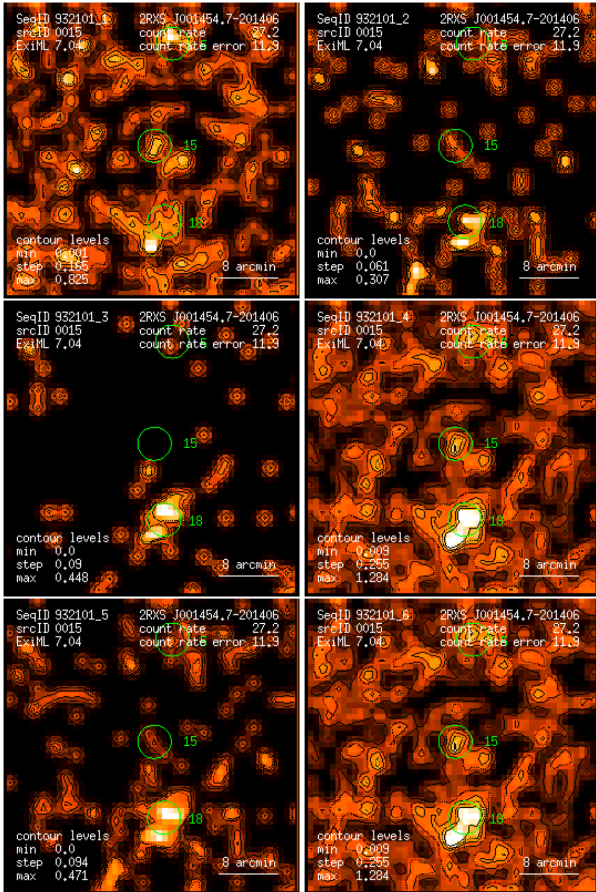
Figure 15: RASS 932101: detection 0015: band rate images, Gaussian filter: (1) PSPC channels 11 – 41, (2) 52 – 90, (3) 91 – 201, (4) 11 – 235, (5) 52 – 201, (6) 11 – 201. Broad band rates in counts/ks. Band rate contour levels in counts/ks/arcmin 2 .
