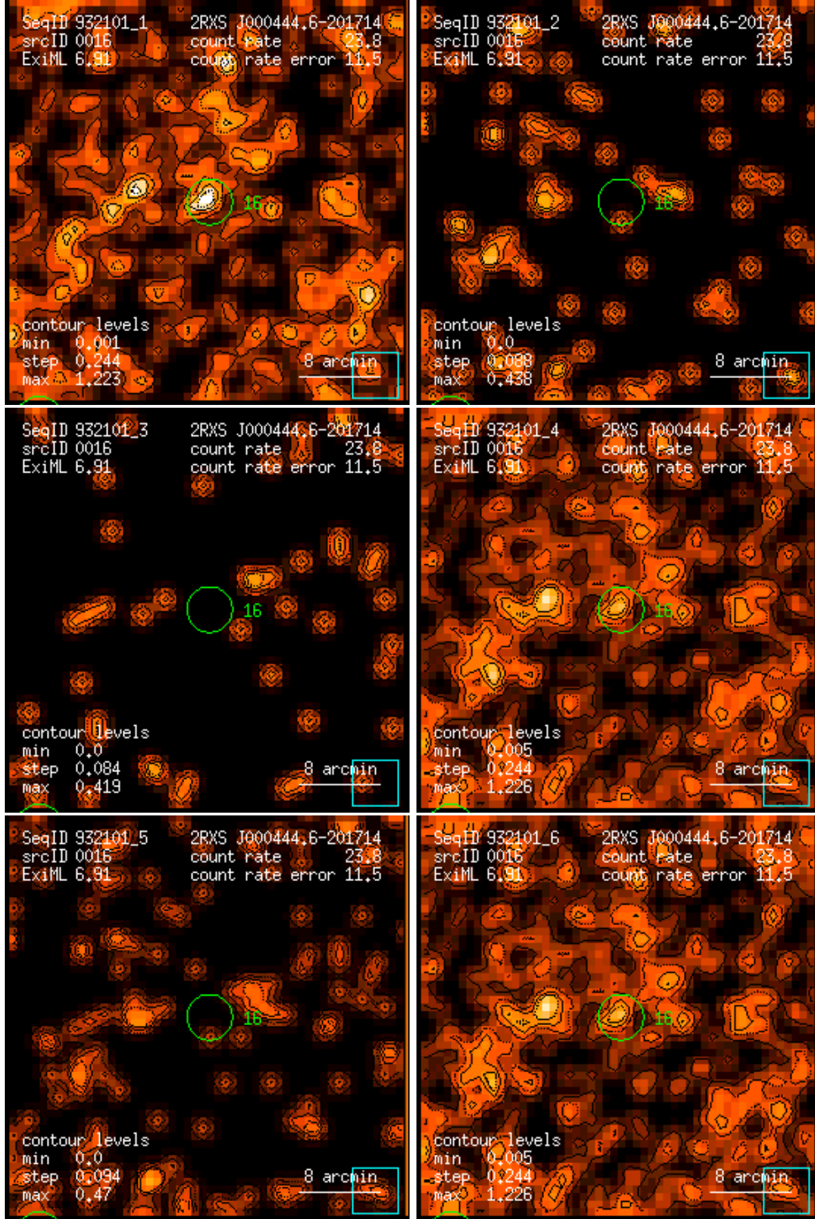
Figure 16: RASS 932101: detection 0016: band rate images, Gaussian filter: (1) PSPC channels 11 – 41, (2) 52 – 90, (3) 91 – 201, (4) 11 – 235, (5) 52 – 201, (6) 11 – 201. Broad band rates in counts/ks. Band rate contour levels in counts/ks/arcmin 2 .
