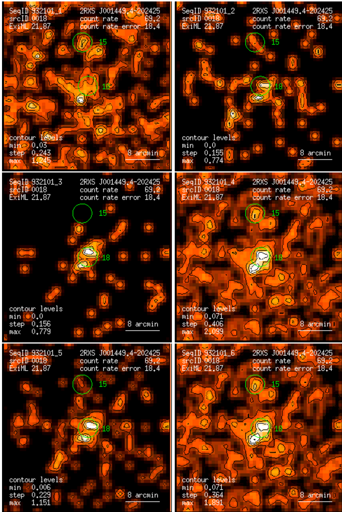
Figure 18: RASS 932101: detection 0018: band rate images, Gaussian filter: (1) PSPC channels 11 – 41, (2) 52 – 90, (3) 91 – 201, (4) 11 – 235, (5) 52 – 201, (6) 11 – 201. Broad band rates in counts/ks. Band rate contour levels in counts/ks/arcmin 2 .
