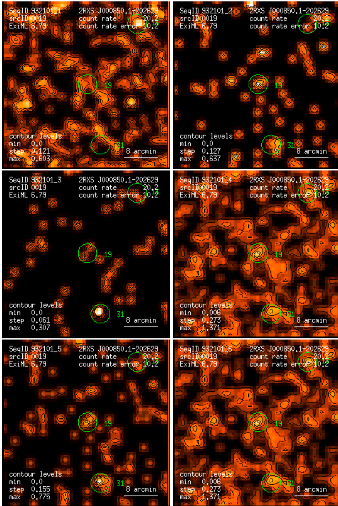
Figure 19: RASS 932101: detection 0019: band rate images, Gaussian filter: (1) PSPC channels 11 – 41, (2) 52 – 90, (3) 91 – 201, (4) 11 – 235, (5) 52 – 201, (6) 11 – 201. Broad band rates in counts/ks. Band rate contour levels in counts/ks/arcmin 2 .
