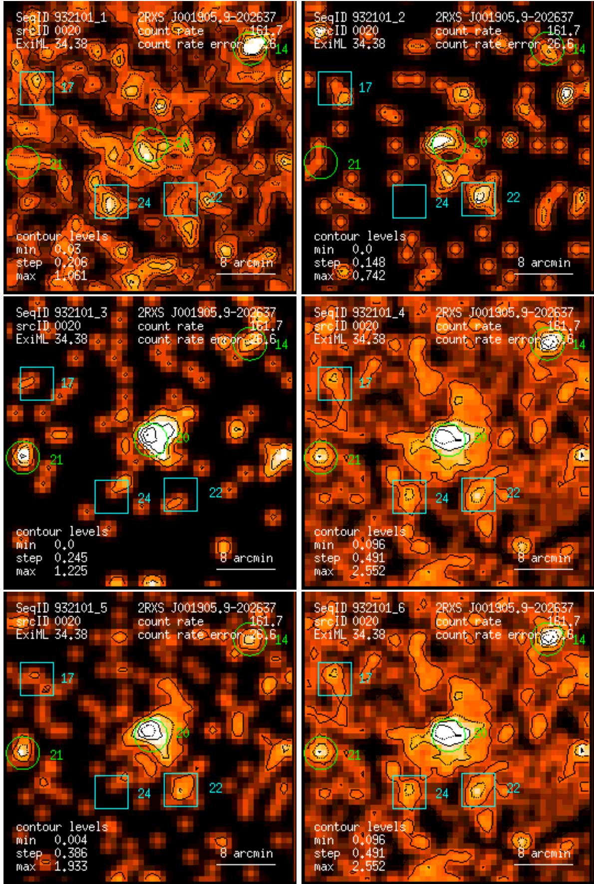
Figure 20: RASS 932101: detection 0020: band rate images, Gaussian filter: (1) PSPC channels 11 – 41, (2) 52 – 90, (3) 91 – 201, (4) 11 – 235, (5) 52 – 201, (6) 11 – 201. Broad band rates in counts/ks. Band rate contour levels in counts/ks/arcmin 2 .
