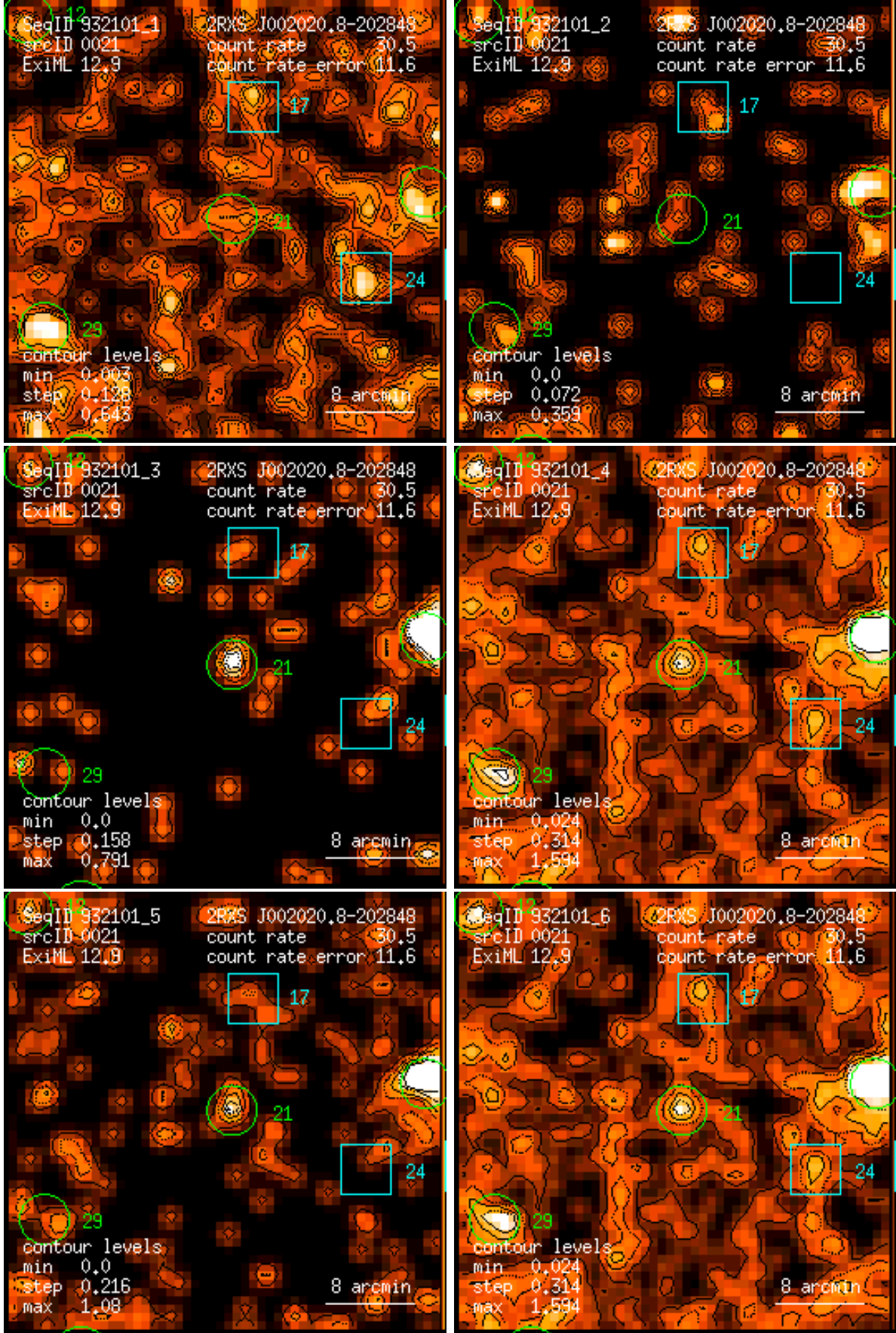
Figure 21: RASS 932101: detection 0021: band rate images, Gaussian filter: (1) PSPC channels 11 – 41, (2) 52 – 90, (3) 91 – 201, (4) 11 – 235, (5) 52 – 201, (6) 11 – 201. Broad band rates in counts/ks. Band rate contour levels in counts/ks/arcmin 2 .
