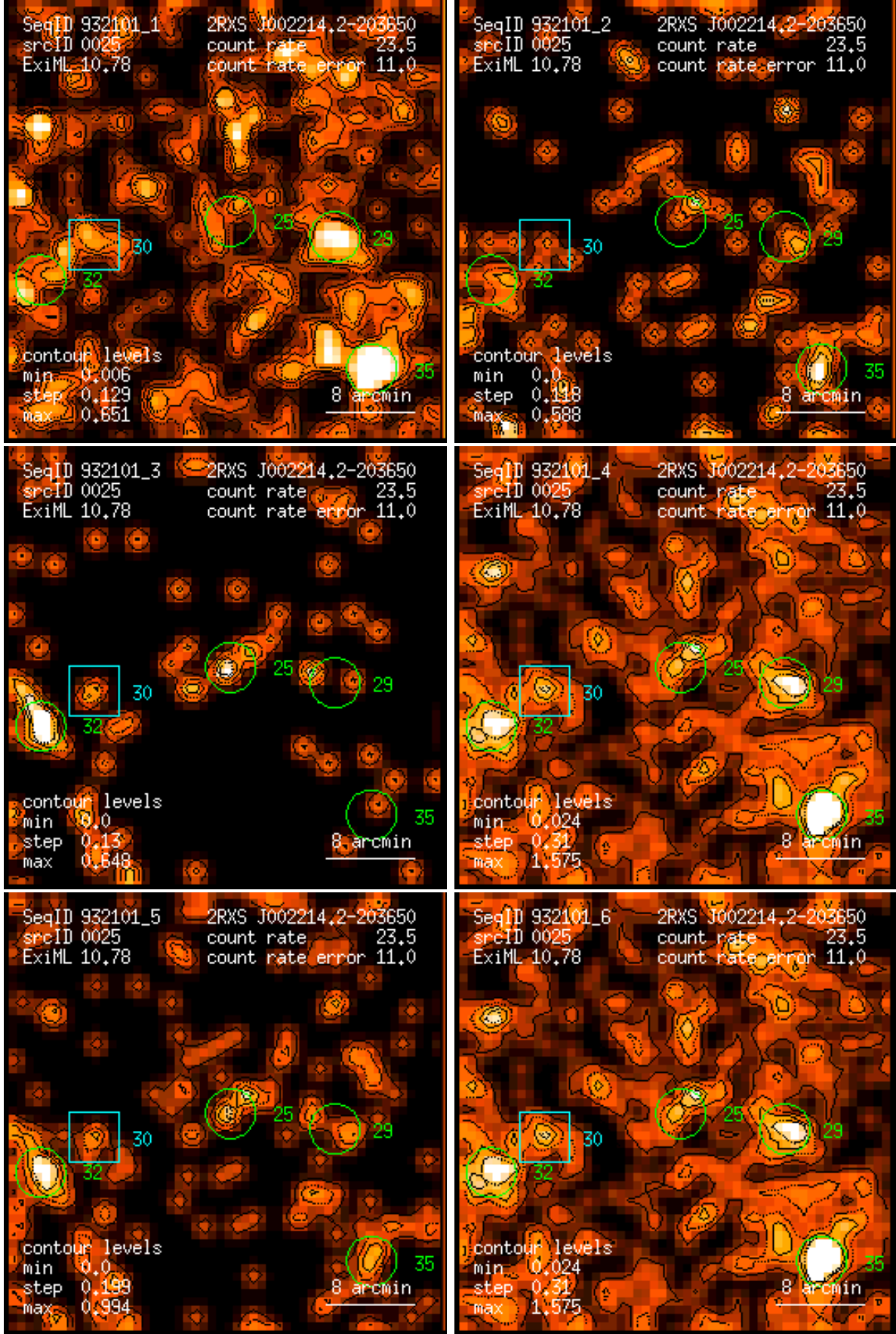
Figure 25: RASS 932101: detection 0025: band rate images, Gaussian filter: (1) PSPC channels 11 – 41, (2) 52 – 90, (3) 91 – 201, (4) 11 – 235, (5) 52 – 201, (6) 11 – 201. Broad band rates in counts/ks. Band rate contour levels in counts/ks/arcmin 2 .
