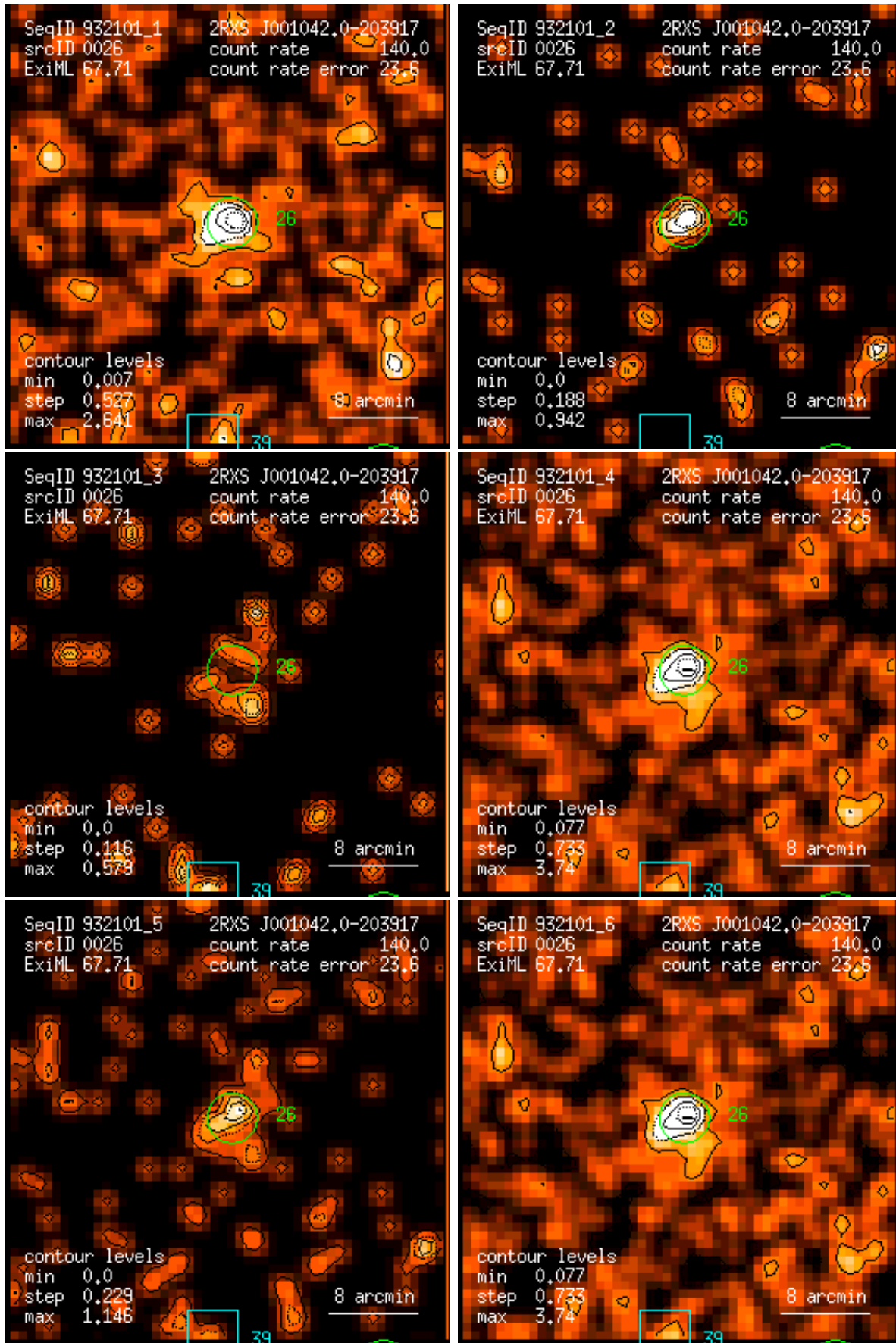
Figure 26: RASS 932101: detection 0026: band rate images, Gaussian filter: (1) PSPC channels 11 – 41, (2) 52 – 90, (3) 91 – 201, (4) 11 – 235, (5) 52 – 201, (6) 11 – 201. Broad band rates in counts/ks. Band rate contour levels in counts/ks/arcmin 2 .
