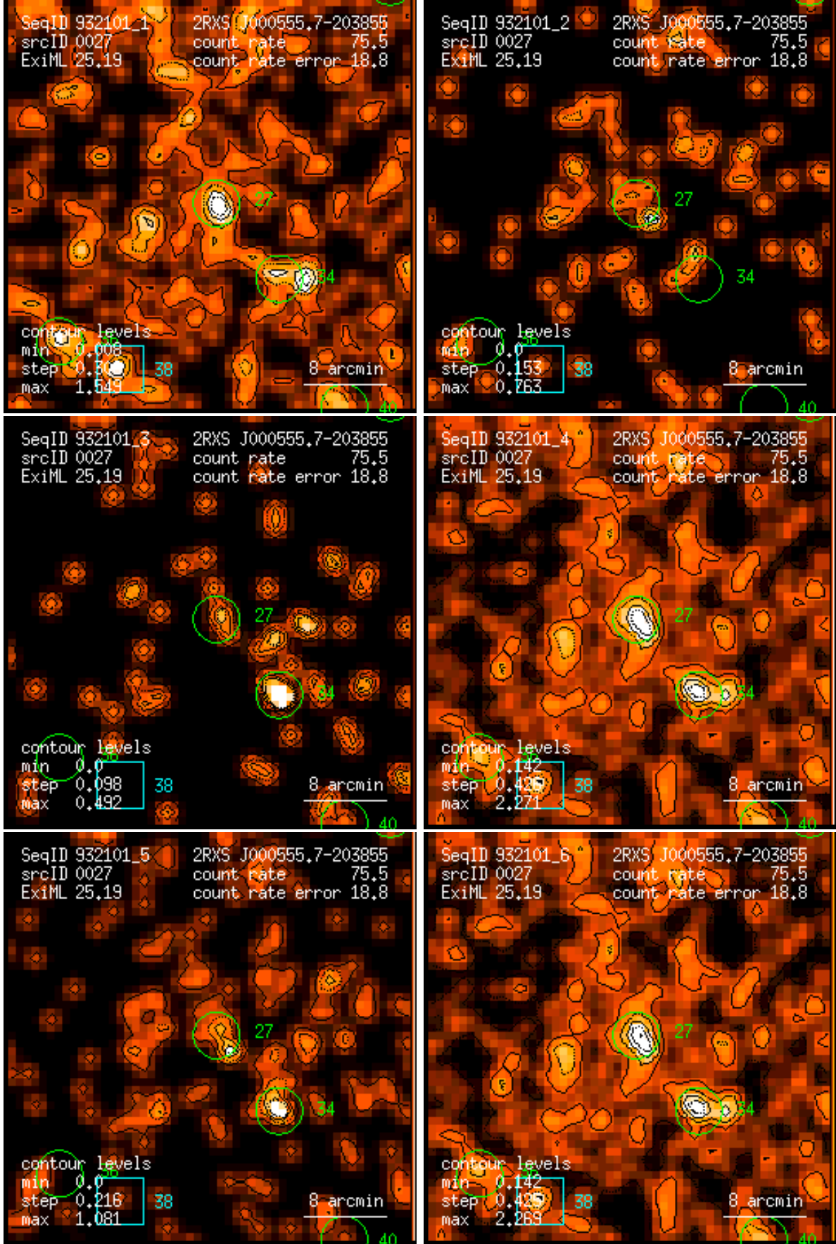
Figure 27: RASS 932101: detection 0027: band rate images, Gaussian filter: (1) PSPC channels 11 – 41, (2) 52 – 90, (3) 91 – 201, (4) 11 – 235, (5) 52 – 201, (6) 11 – 201. Broad band rates in counts/ks. Band rate contour levels in counts/ks/arcmin 2 .
