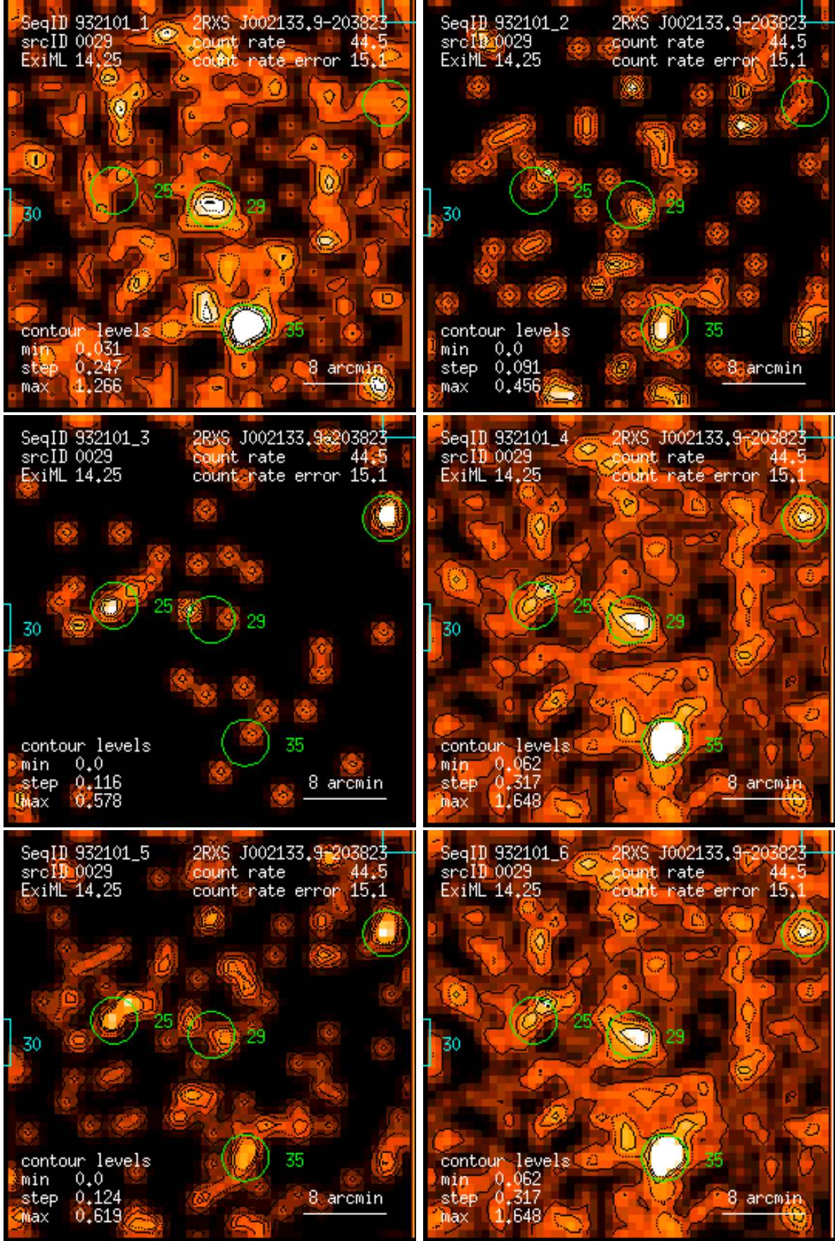
Figure 29: RASS 932101: detection 0029: band rate images, Gaussian filter: (1) PSPC channels 11 – 41, (2) 52 – 90, (3) 91 – 201, (4) 11 – 235, (5) 52 – 201, (6) 11 – 201. Broad band rates in counts/ks. Band rate contour levels in counts/ks/arcmin 2 .
